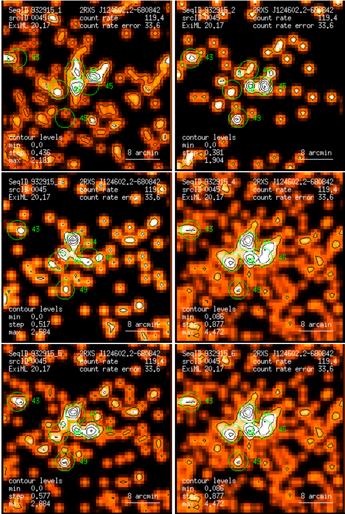
Figure 45: RASS 932915: detection 0045: band rate images, Gaussian filter: (1) PSPC channels 11 – 41, (2) 52 – 90, (3) 91 – 201, (4) 11 – 235, (5) 52 – 201, (6) 11 – 201. Broad band rates in counts/ks. Band rate contour levels in counts/ks/arcmin 2 .
