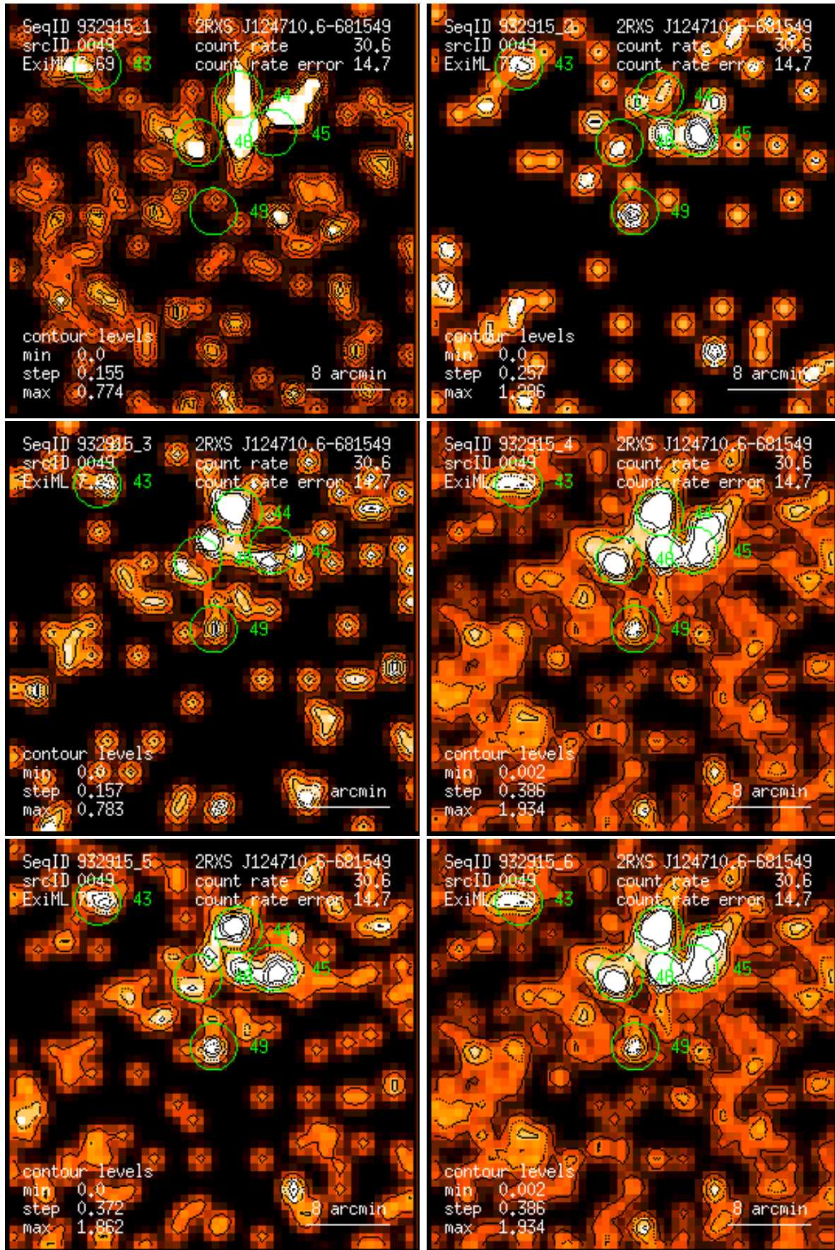
Figure 49: RASS 932915: detection 0049: band rate images, Gaussian filter: (1) PSPC channels 11 – 41, (2) 52 – 90, (3) 91 – 201, (4) 11 – 235, (5) 52 – 201, (6) 11 – 201. Broad band rates in counts/ks. Band rate contour levels in counts/ks/arcmin 2 .
