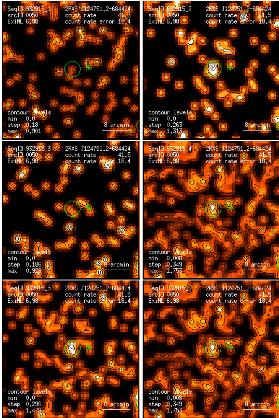
Figure 50: RASS 932915: detection 0050: band rate images, Gaussian filter: (1) PSPC channels 11 – 41, (2) 52 – 90, (3) 91 – 201, (4) 11 – 235, (5) 52 – 201, (6) 11 – 201. Broad band rates in counts/ks. Band rate contour levels in counts/ks/arcmin 2 .
