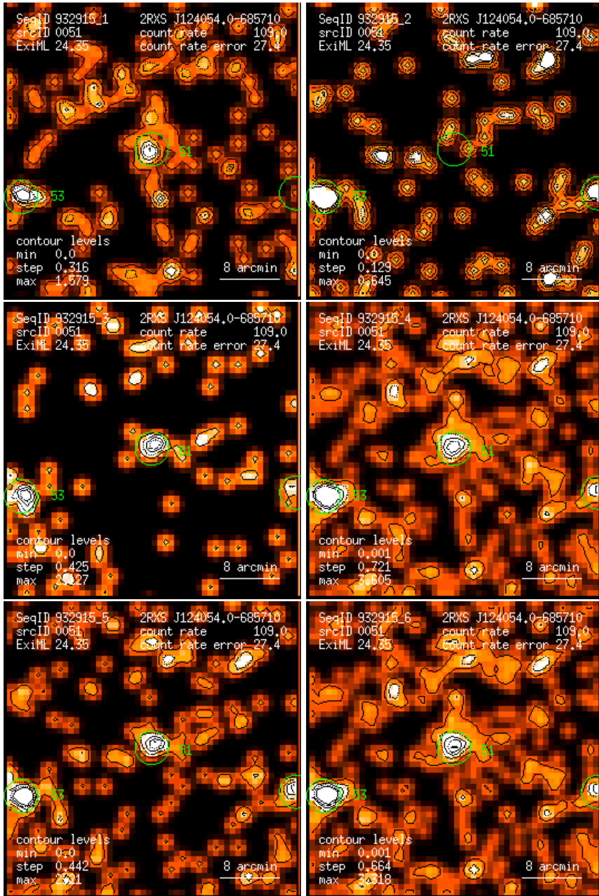
Figure 51: RASS 932915: detection 0051: band rate images, Gaussian filter: (1) PSPC channels 11 – 41, (2) 52 – 90, (3) 91 – 201, (4) 11 – 235, (5) 52 – 201, (6) 11 – 201. Broad band rates in counts/ks. Band rate contour levels in counts/ks/arcmin 2 .
