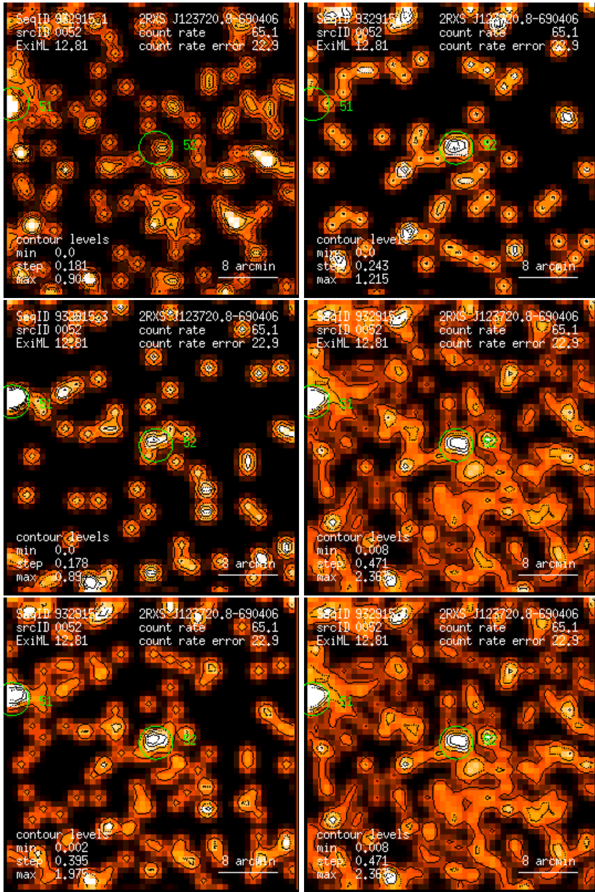
Figure 52: RASS 932915: detection 0052: band rate images, Gaussian filter: (1) PSPC channels 11 – 41, (2) 52 – 90, (3) 91 – 201, (4) 11 – 235, (5) 52 – 201, (6) 11 – 201. Broad band rates in counts/ks. Band rate contour levels in counts/ks/arcmin 2 .
