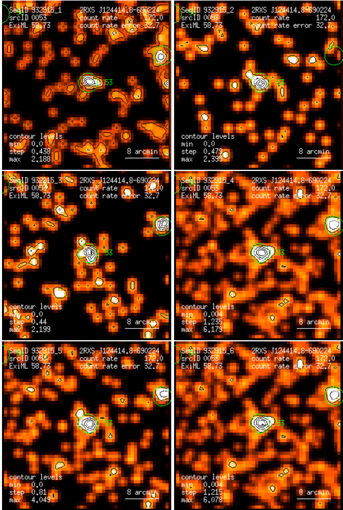
Figure 53: RASS 932915: detection 0053: band rate images, Gaussian filter: (1) PSPC channels 11 – 41, (2) 52 – 90, (3) 91 – 201, (4) 11 – 235, (5) 52 – 201, (6) 11 – 201. Broad band rates in counts/ks. Band rate contour levels in counts/ks/arcmin 2 .
