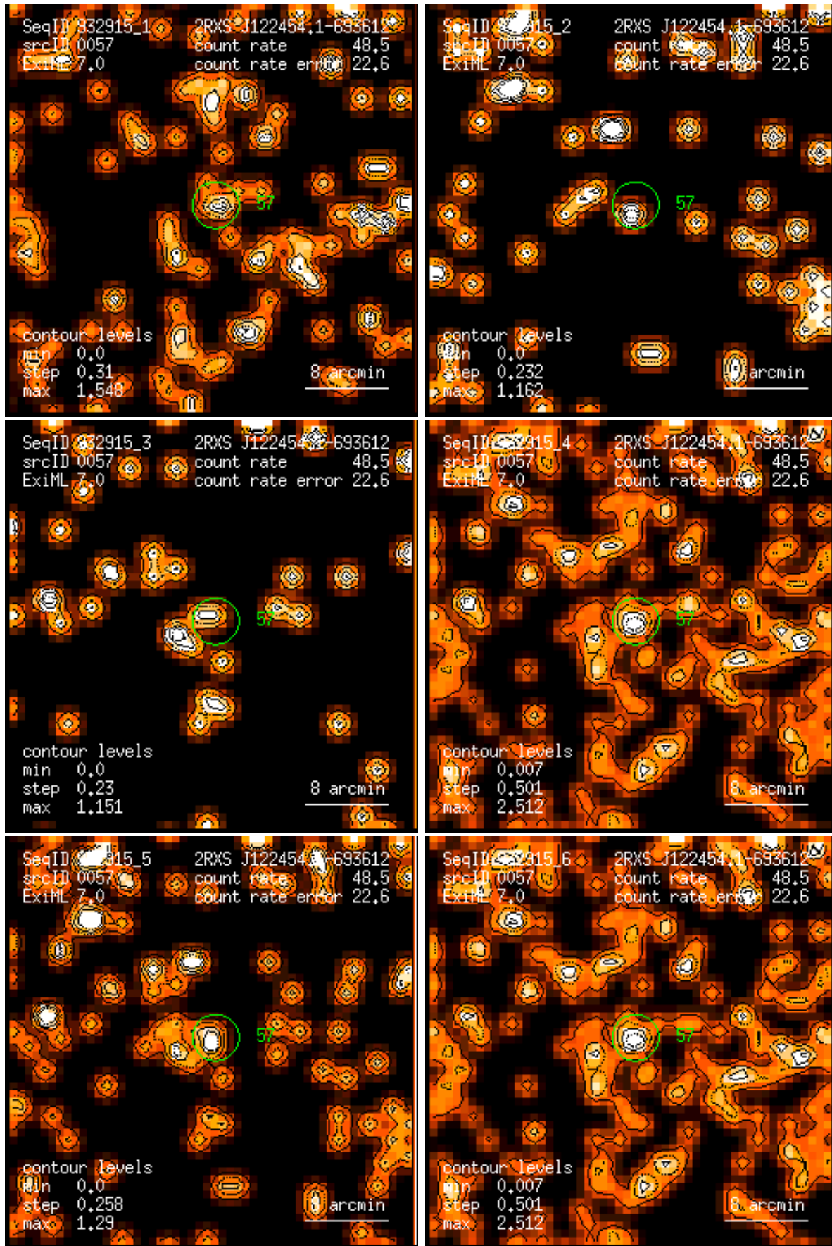
Figure 57: RASS 932915: detection 0057: band rate images, Gaussian filter: (1) PSPC channels 11 – 41, (2) 52 – 90, (3) 91 – 201, (4) 11 – 235, (5) 52 – 201, (6) 11 – 201. Broad band rates in counts/ks. Band rate contour levels in counts/ks/arcmin 2 .
