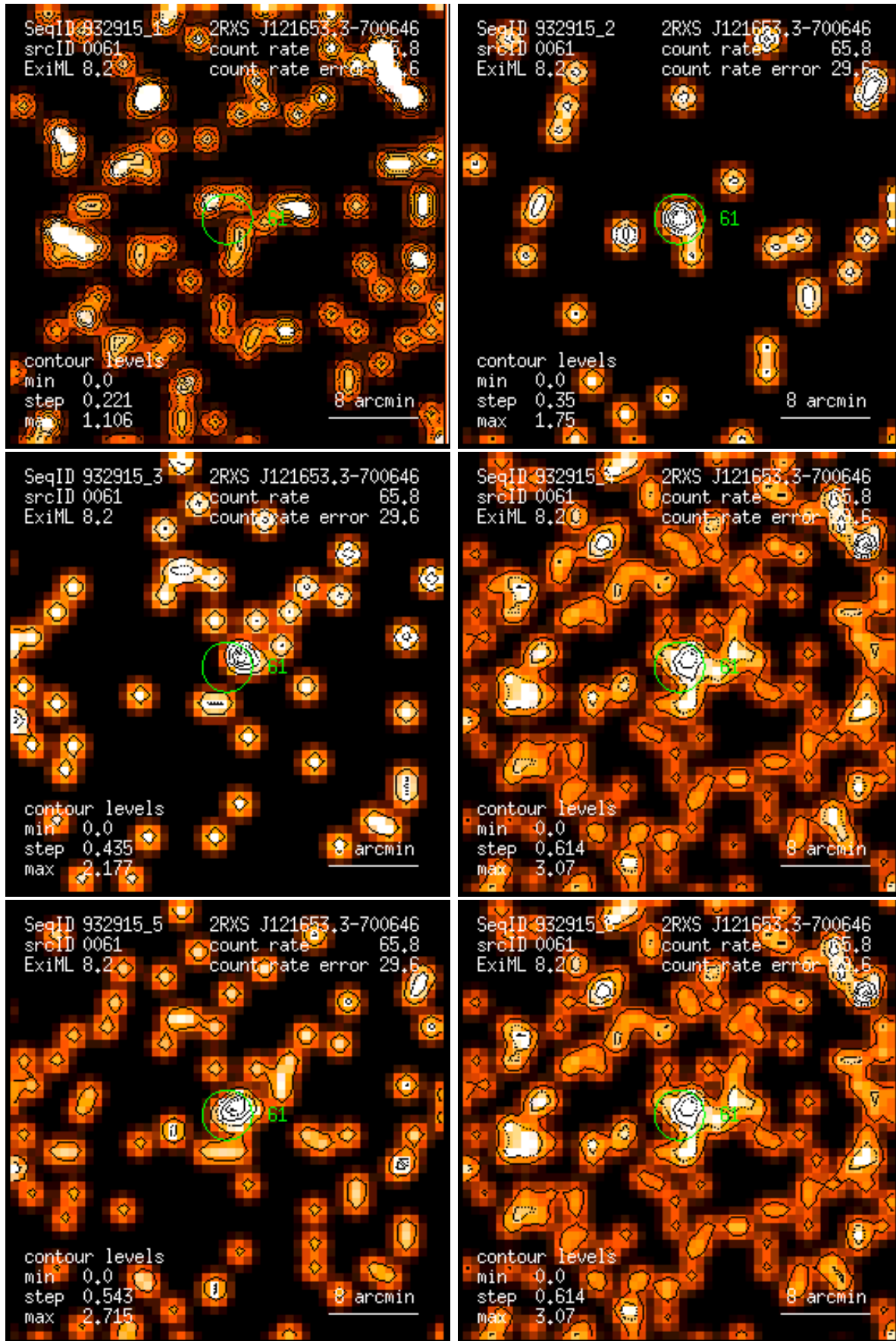
Figure 61: RASS 932915: detection 0061: band rate images, Gaussian filter: (1) PSPC channels 11 – 41, (2) 52 – 90, (3) 91 – 201, (4) 11 – 235, (5) 52 – 201, (6) 11 – 201. Broad band rates in counts/ks. Band rate contour levels in counts/ks/arcmin 2 .
