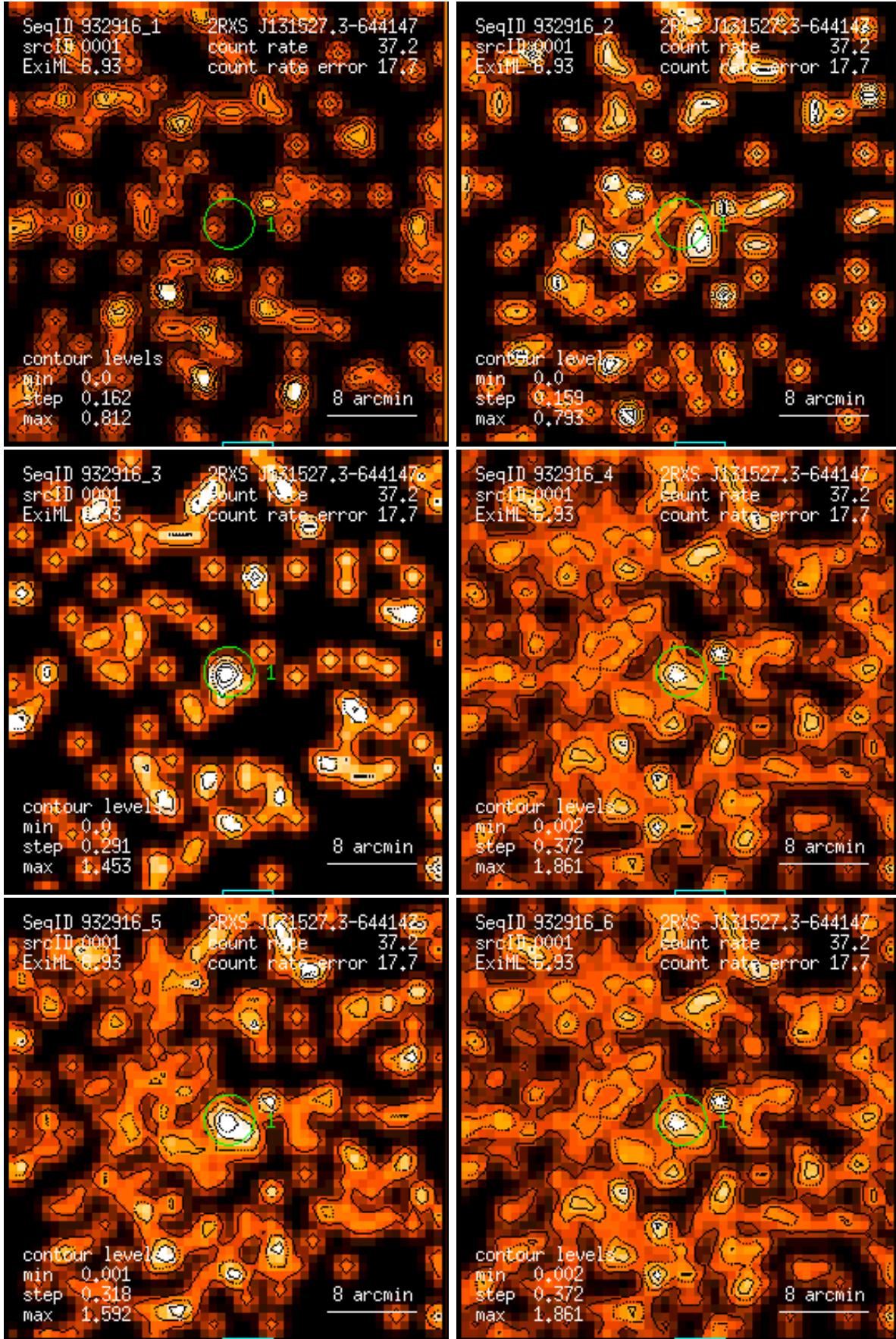
Figure 1: RASS 932916: detection 0001: band rate images, Gaussian filter: (1) PSPC channels 11 – 41, (2) 52 – 90, (3) 91 – 201, (4) 11 – 235, (5) 52 – 201, (6) 11 – 201. Broad band rates in counts/ks. Band rate contour levels in counts/ks/arcmin 2 .
