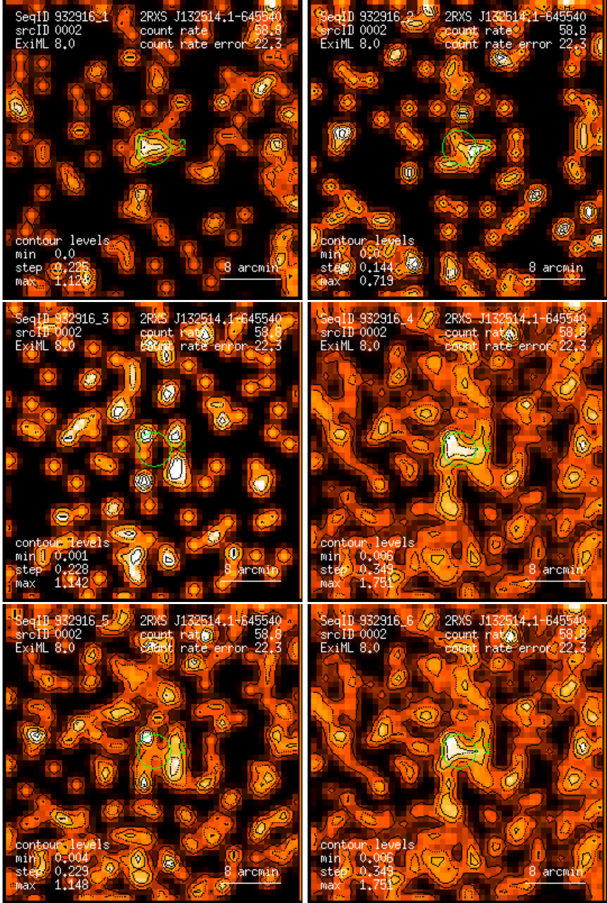
Figure 2: RASS 932916: detection 0002: band rate images, Gaussian filter: (1) PSPC channels 11 – 41, (2) 52 – 90, (3) 91 – 201, (4) 11 – 235, (5) 52 – 201, (6) 11 – 201. Broad band rates in counts/ks. Band rate contour levels in counts/ks/arcmin 2 .
