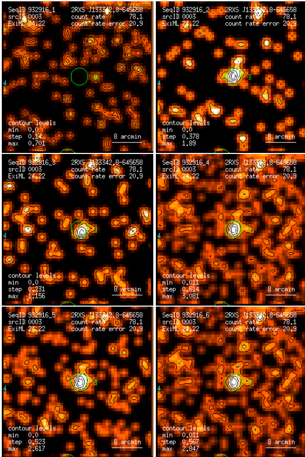
Figure 3: RASS 932916: detection 0003: band rate images, Gaussian filter: (1) PSPC channels 11 – 41, (2) 52 – 90, (3) 91 – 201, (4) 11 – 235, (5) 52 – 201, (6) 11 – 201. Broad band rates in counts/ks. Band rate contour levels in counts/ks/arcmin 2 .
