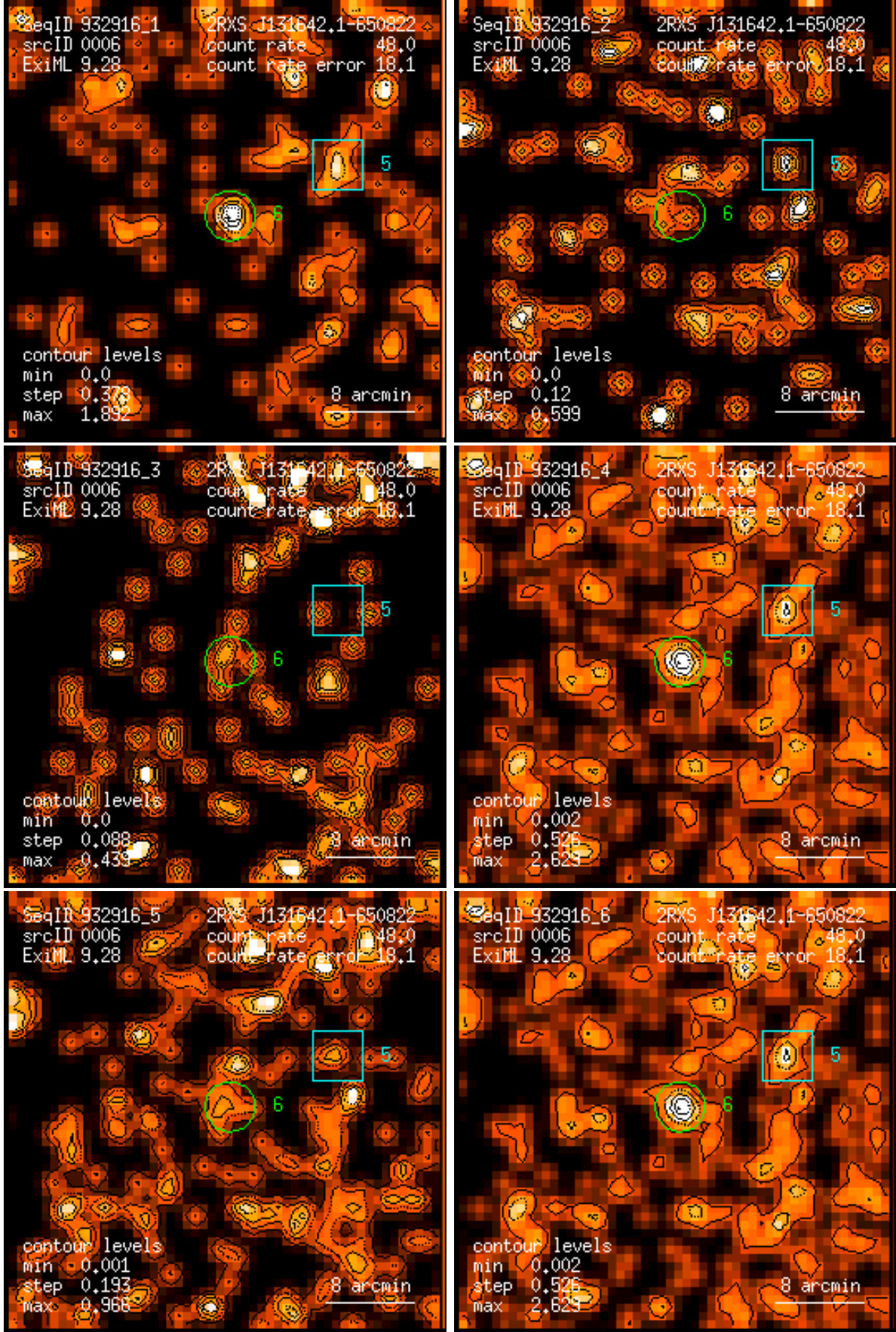
Figure 6: RASS 932916: detection 0006: band rate images, Gaussian filter: (1) PSPC channels 11 – 41, (2) 52 – 90, (3) 91 – 201, (4) 11 – 235, (5) 52 – 201, (6) 11 – 201. Broad band rates in counts/ks. Band rate contour levels in counts/ks/arcmin 2 .
