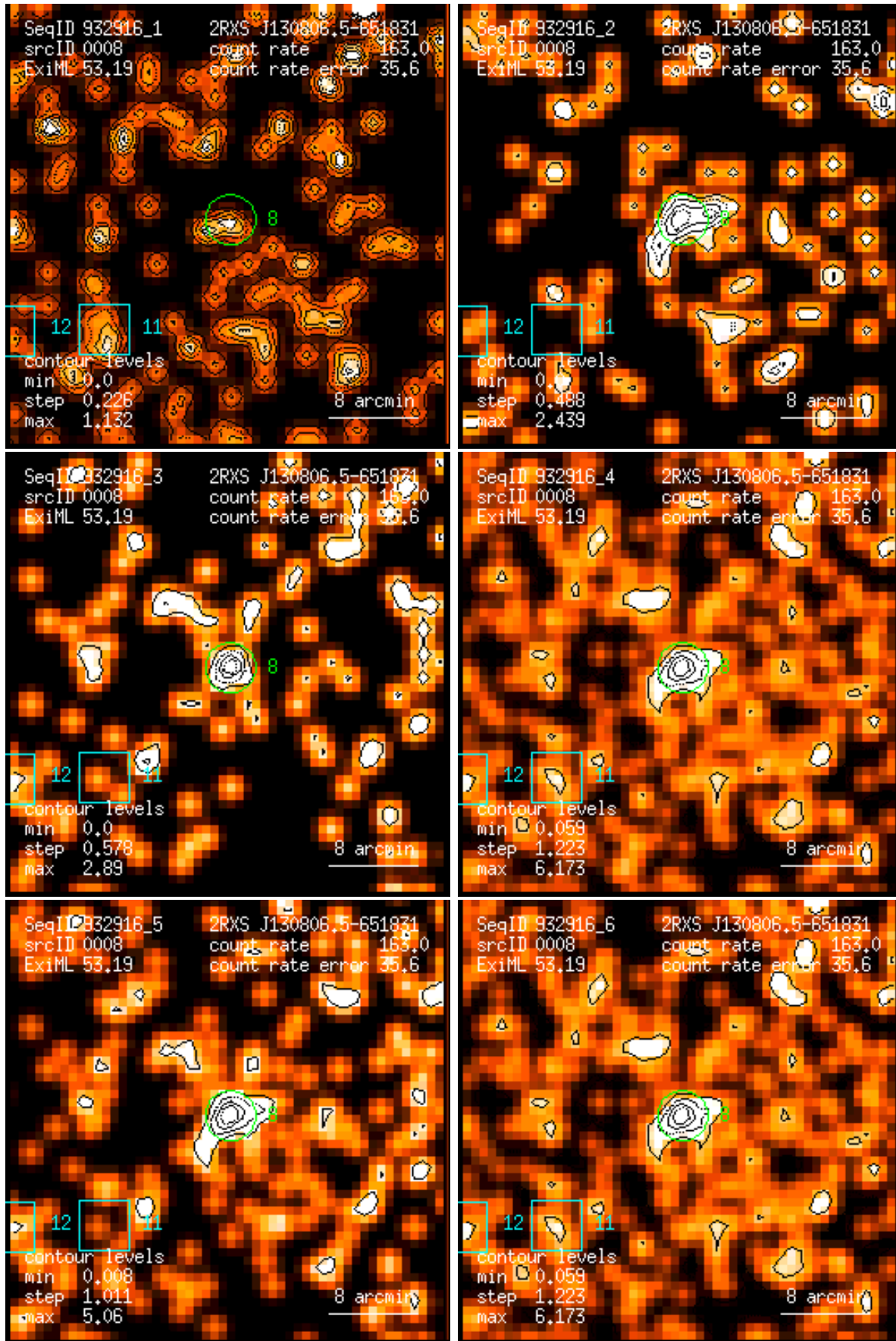
Figure 8: RASS 932916: detection 0008: band rate images, Gaussian filter: (1) PSPC channels 11 – 41, (2) 52 – 90, (3) 91 – 201, (4) 11 – 235, (5) 52 – 201, (6) 11 – 201. Broad band rates in counts/ks. Band rate contour levels in counts/ks/arcmin 2 .
