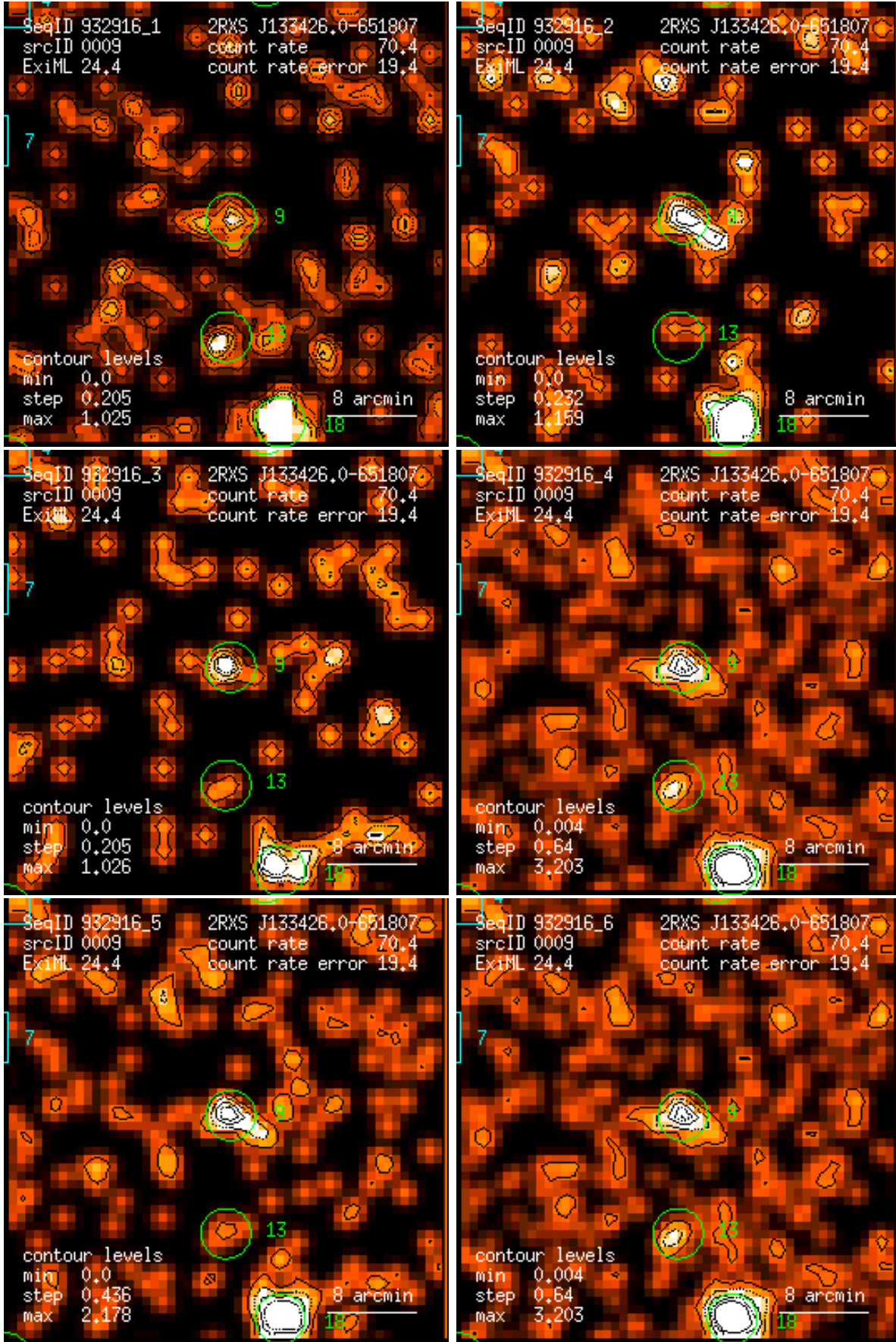
Figure 9: RASS 932916: detection 0009: band rate images, Gaussian filter: (1) PSPC channels 11 – 41, (2) 52 – 90, (3) 91 – 201, (4) 11 – 235, (5) 52 – 201, (6) 11 – 201. Broad band rates in counts/ks. Band rate contour levels in counts/ks/arcmin 2 .
