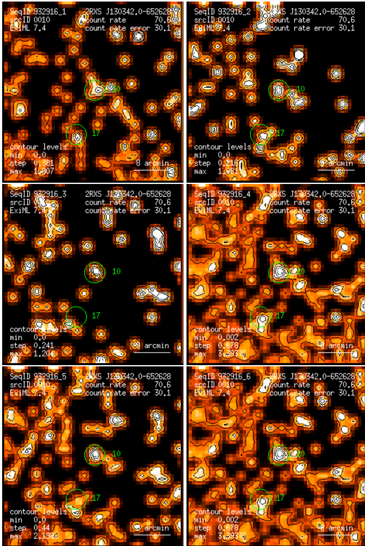
Figure 10: RASS 932916: detection 0010: band rate images, Gaussian filter: (1) PSPC channels 11 – 41, (2) 52 – 90, (3) 91 – 201, (4) 11 – 235, (5) 52 – 201, (6) 11 – 201. Broad band rates in counts/ks. Band rate contour levels in counts/ks/arcmin 2 .
