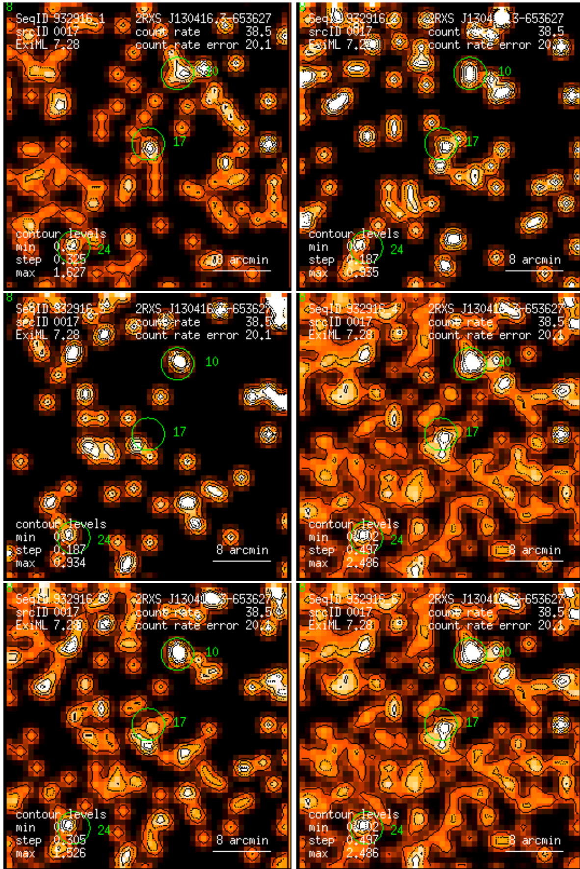
Figure 17: RASS 932916: detection 0017: band rate images, Gaussian filter: (1) PSPC channels 11 – 41, (2) 52 – 90, (3) 91 – 201, (4) 11 – 235, (5) 52 – 201, (6) 11 – 201. Broad band rates in counts/ks. Band rate contour levels in counts/ks/arcmin 2 .
