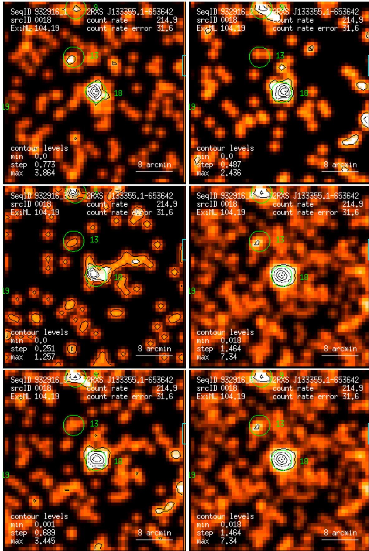
Figure 18: RASS 932916: detection 0018: band rate images, Gaussian filter: (1) PSPC channels 11 – 41, (2) 52 – 90, (3) 91 – 201, (4) 11 – 235, (5) 52 – 201, (6) 11 – 201. Broad band rates in counts/ks. Band rate contour levels in counts/ks/arcmin 2 .
