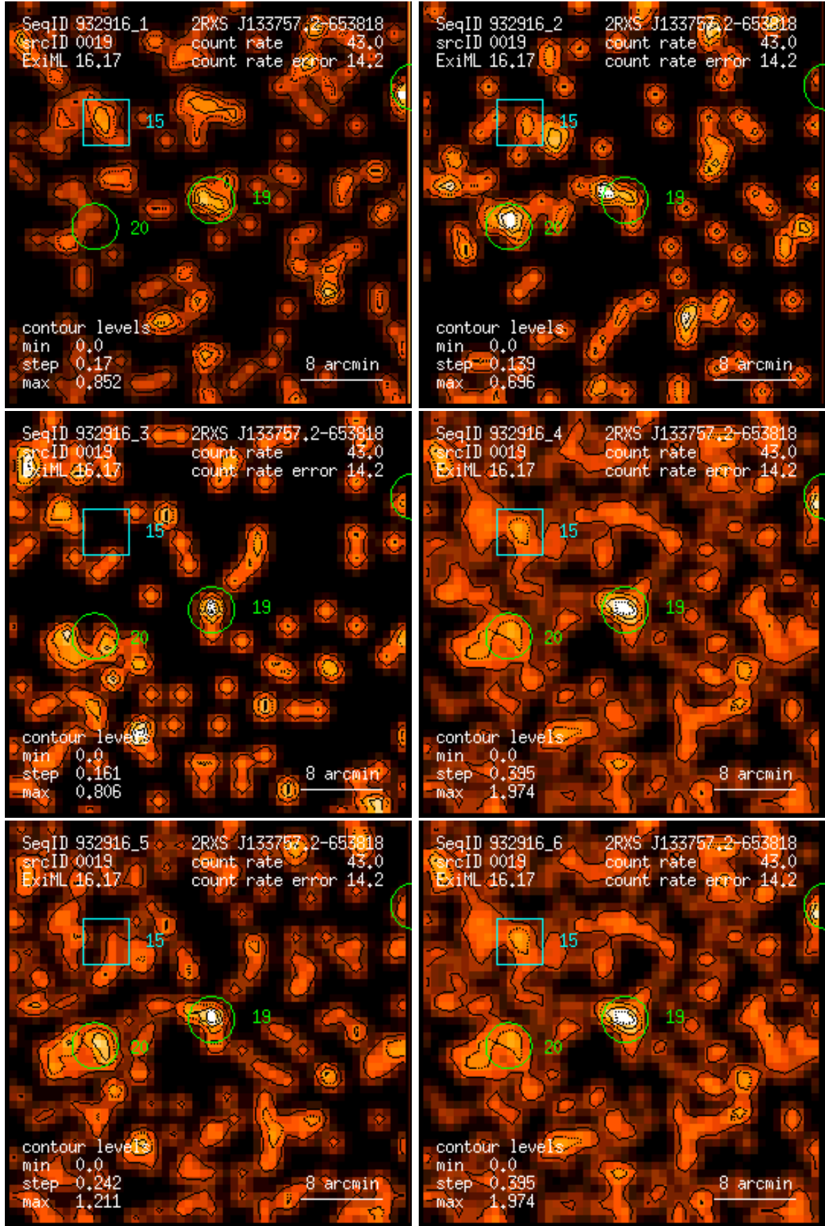
Figure 19: RASS 932916: detection 0019: band rate images, Gaussian filter: (1) PSPC channels 11 – 41, (2) 52 – 90, (3) 91 – 201, (4) 11 – 235, (5) 52 – 201, (6) 11 – 201. Broad band rates in counts/ks. Band rate contour levels in counts/ks/arcmin 2 .
