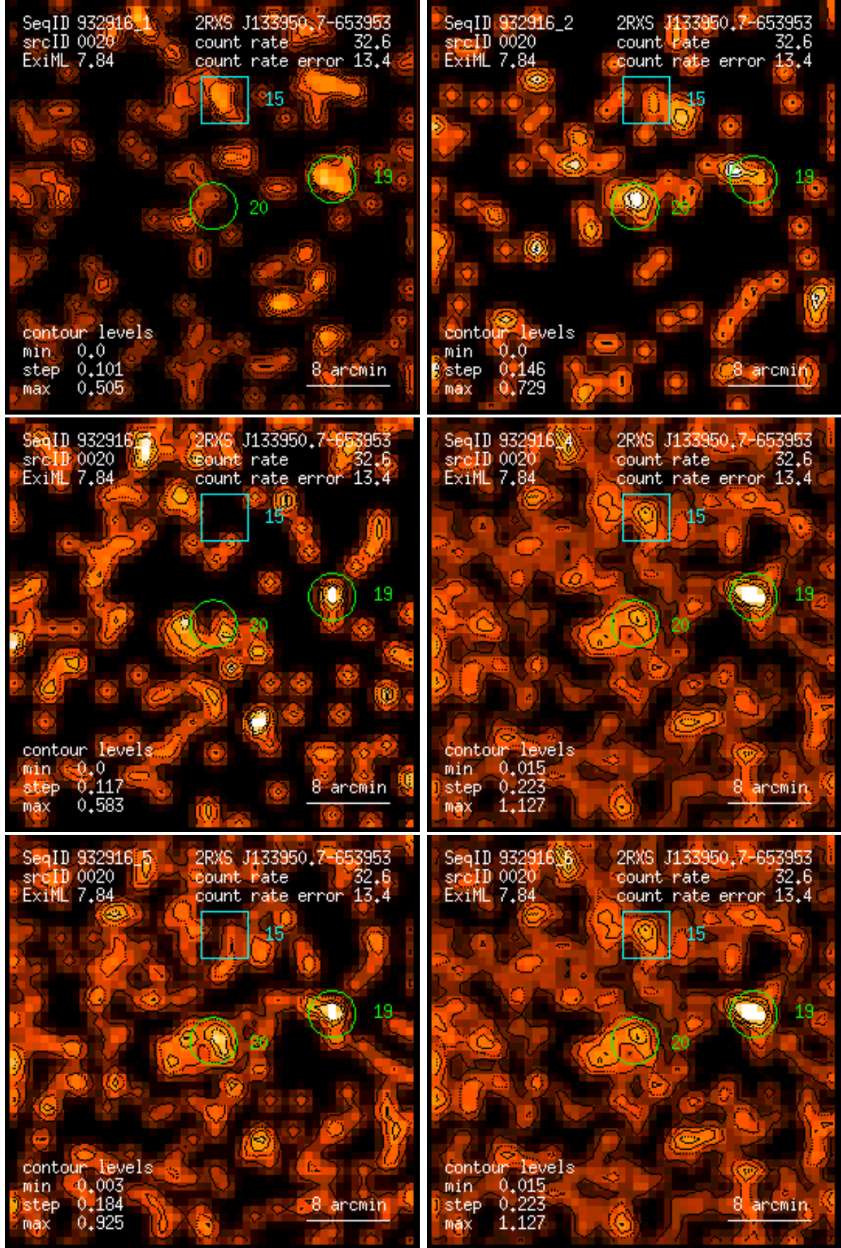
Figure 20: RASS 932916: detection 0020: band rate images, Gaussian filter: (1) PSPC channels 11 – 41, (2) 52 – 90, (3) 91 – 201, (4) 11 – 235, (5) 52 – 201, (6) 11 – 201. Broad band rates in counts/ks. Band rate contour levels in counts/ks/arcmin 2 .
