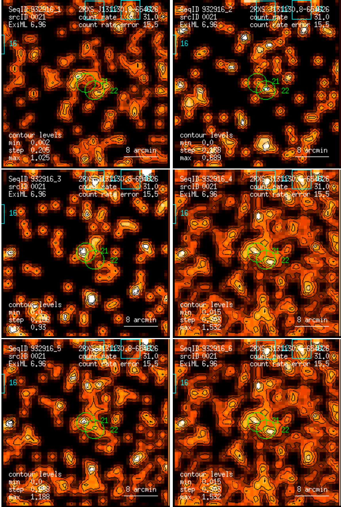
Figure 21: RASS 932916: detection 0021: band rate images, Gaussian filter: (1) PSPC channels 11 – 41, (2) 52 – 90, (3) 91 – 201, (4) 11 – 235, (5) 52 – 201, (6) 11 – 201. Broad band rates in counts/ks. Band rate contour levels in counts/ks/arcmin 2 .
