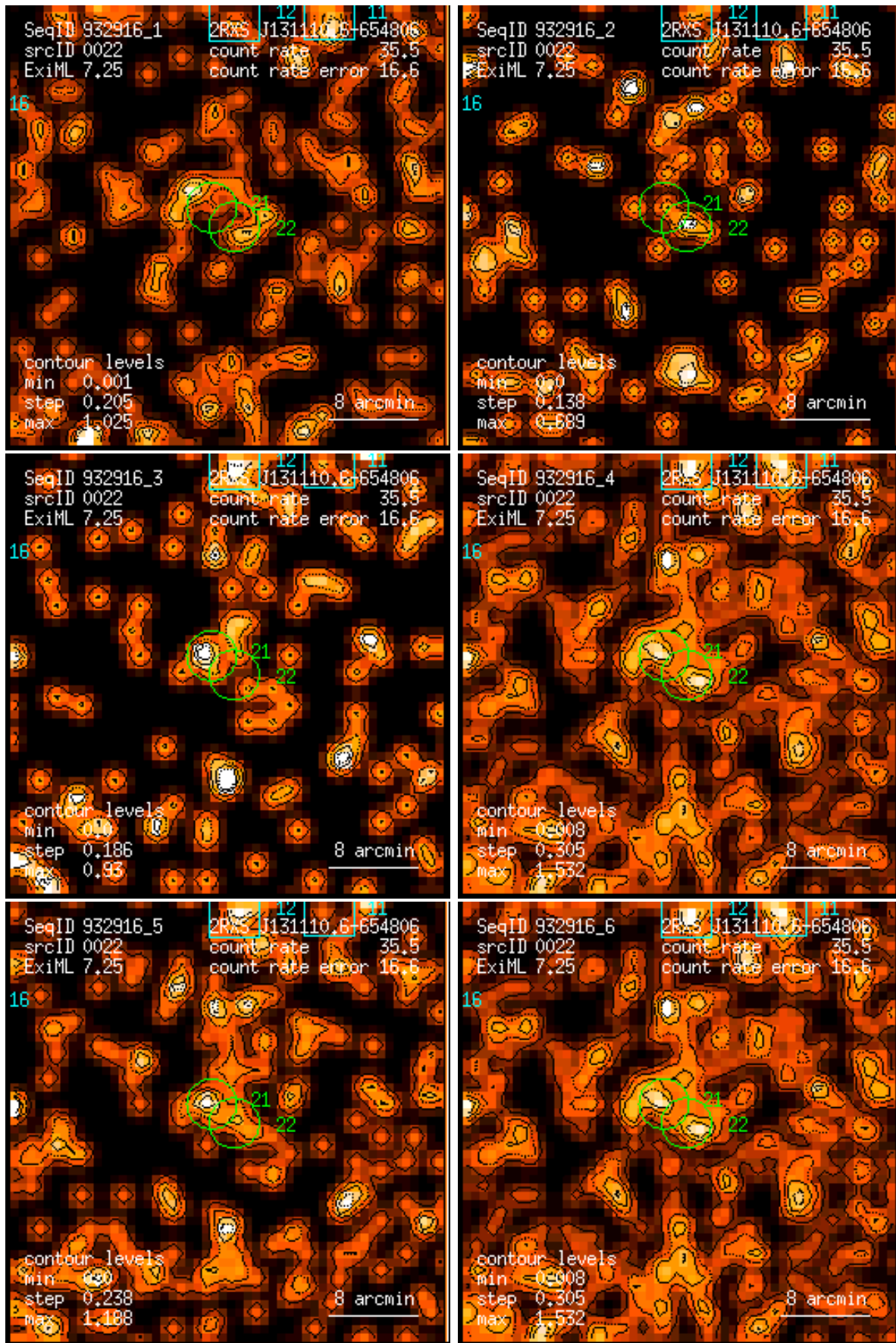
Figure 22: RASS 932916: detection 0022: band rate images, Gaussian filter: (1) PSPC channels 11 – 41, (2) 52 – 90, (3) 91 – 201, (4) 11 – 235, (5) 52 – 201, (6) 11 – 201. Broad band rates in counts/ks. Band rate contour levels in counts/ks/arcmin 2 .
