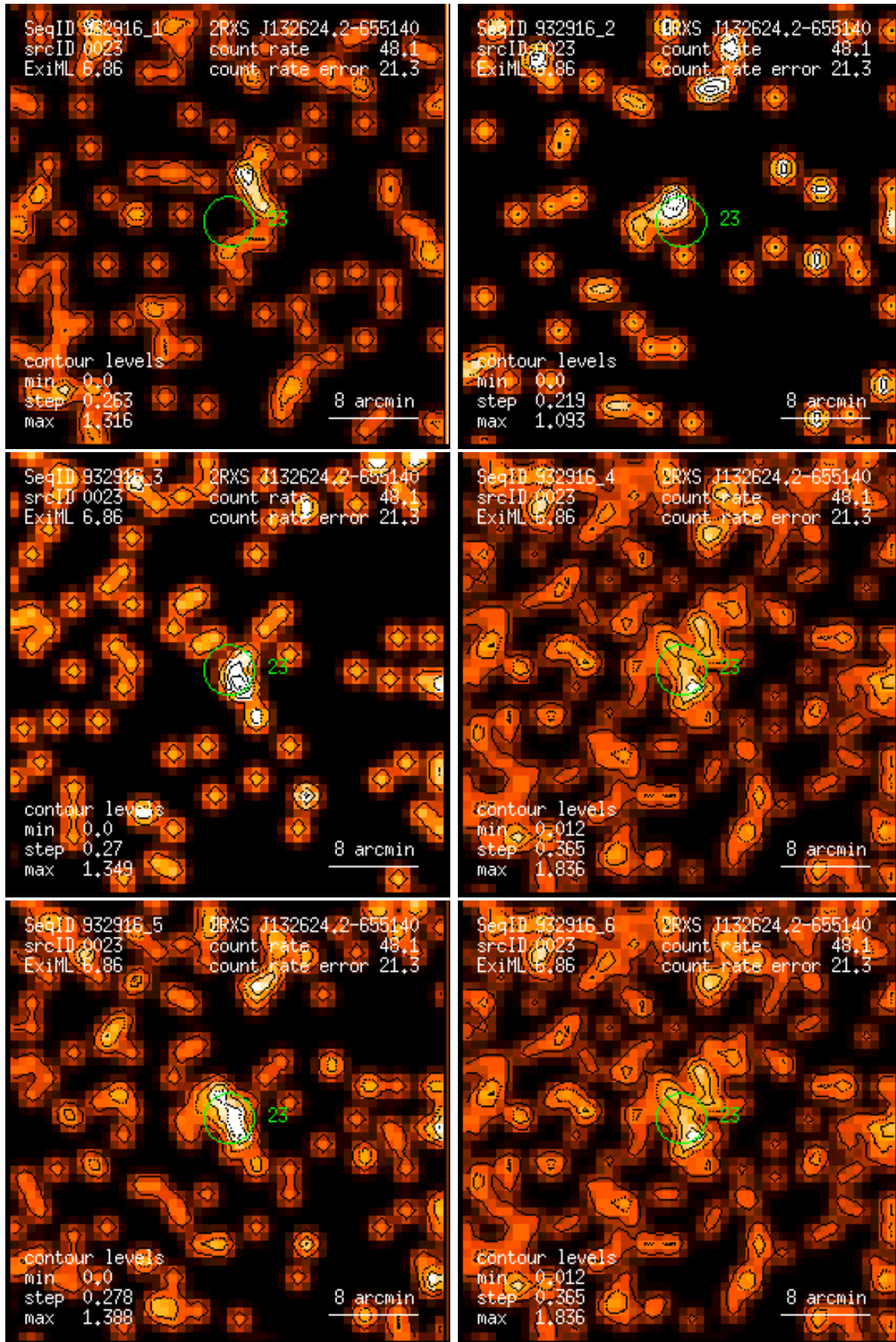
Figure 23: RASS 932916: detection 0023: band rate images, Gaussian filter: (1) PSPC channels 11 – 41, (2) 52 – 90, (3) 91 – 201, (4) 11 – 235, (5) 52 – 201, (6) 11 – 201. Broad band rates in counts/ks. Band rate contour levels in counts/ks/arcmin 2 .
