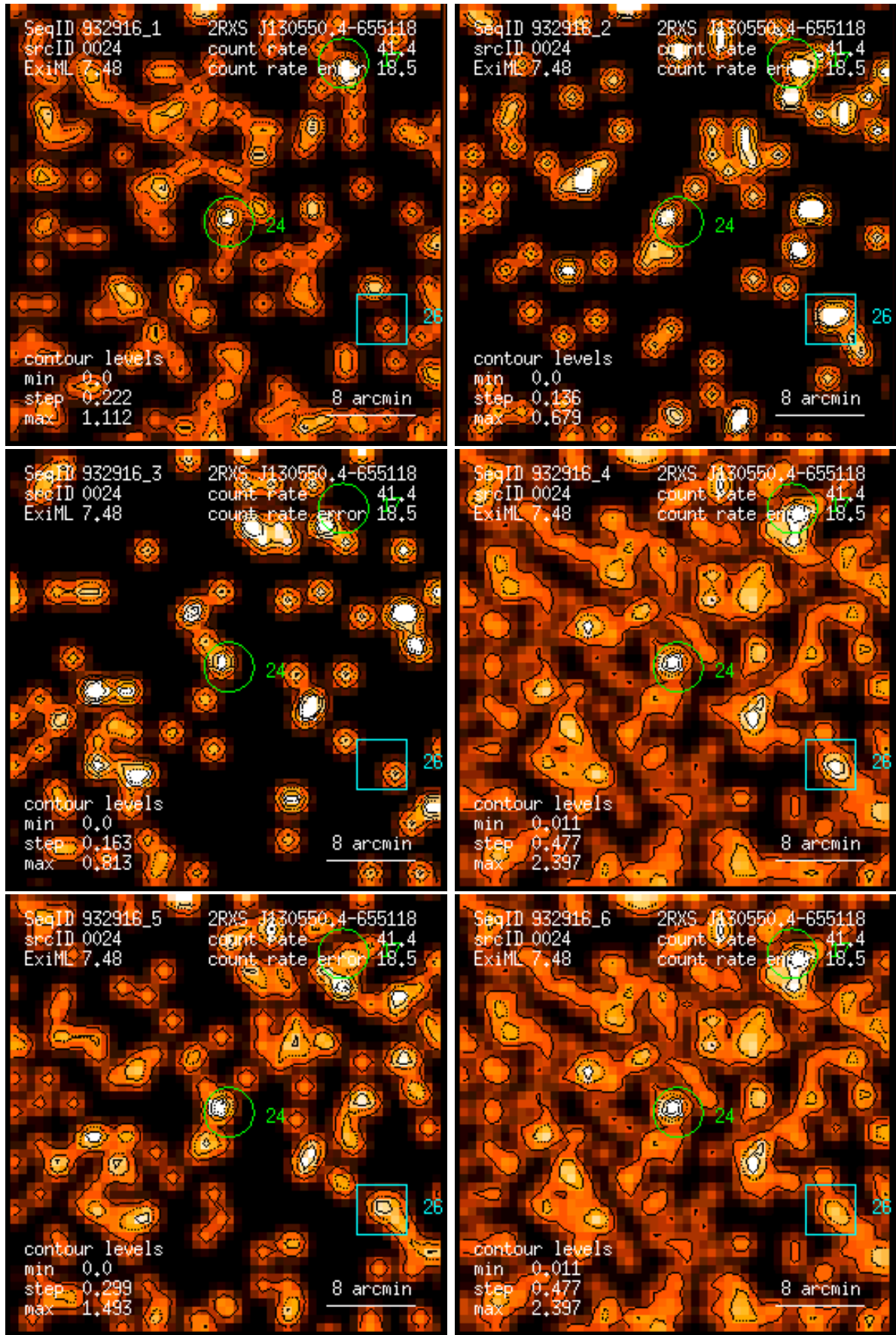
Figure 24: RASS 932916: detection 0024: band rate images, Gaussian filter: (1) PSPC channels 11 – 41, (2) 52 – 90, (3) 91 – 201, (4) 11 – 235, (5) 52 – 201, (6) 11 – 201. Broad band rates in counts/ks. Band rate contour levels in counts/ks/arcmin 2 .
