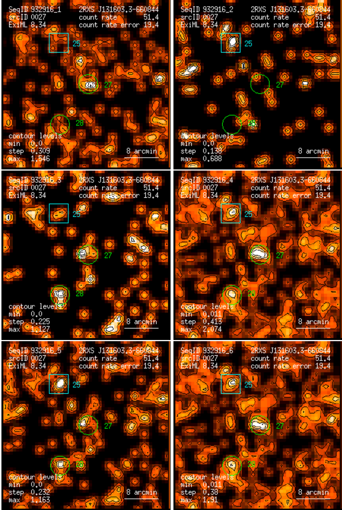
Figure 27: RASS 932916: detection 0027: band rate images, Gaussian filter: (1) PSPC channels 11 – 41, (2) 52 – 90, (3) 91 – 201, (4) 11 – 235, (5) 52 – 201, (6) 11 – 201. Broad band rates in counts/ks. Band rate contour levels in counts/ks/arcmin 2 .
