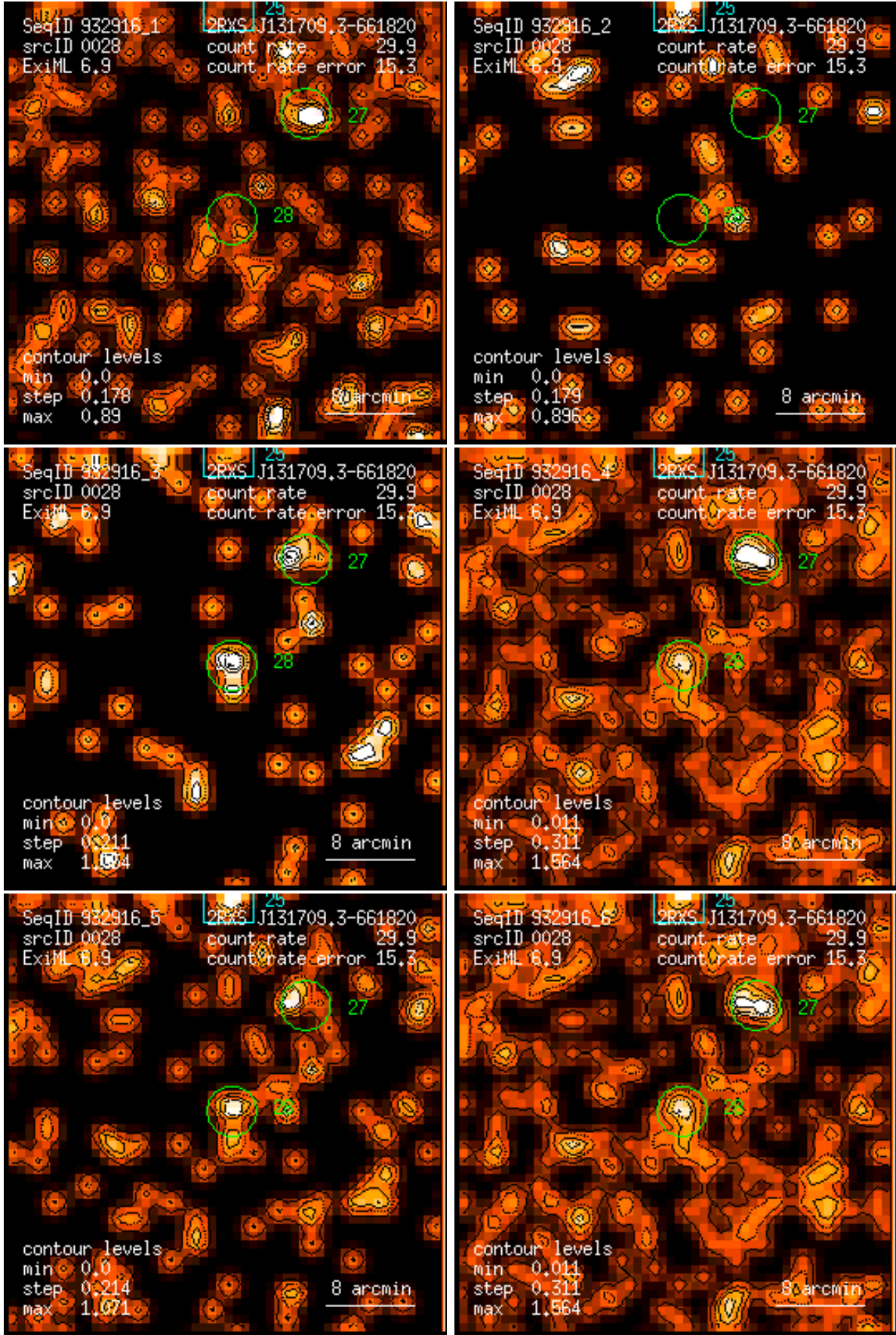
Figure 28: RASS 932916: detection 0028: band rate images, Gaussian filter: (1) PSPC channels 11 – 41, (2) 52 – 90, (3) 91 – 201, (4) 11 – 235, (5) 52 – 201, (6) 11 – 201. Broad band rates in counts/ks. Band rate contour levels in counts/ks/arcmin 2 .
