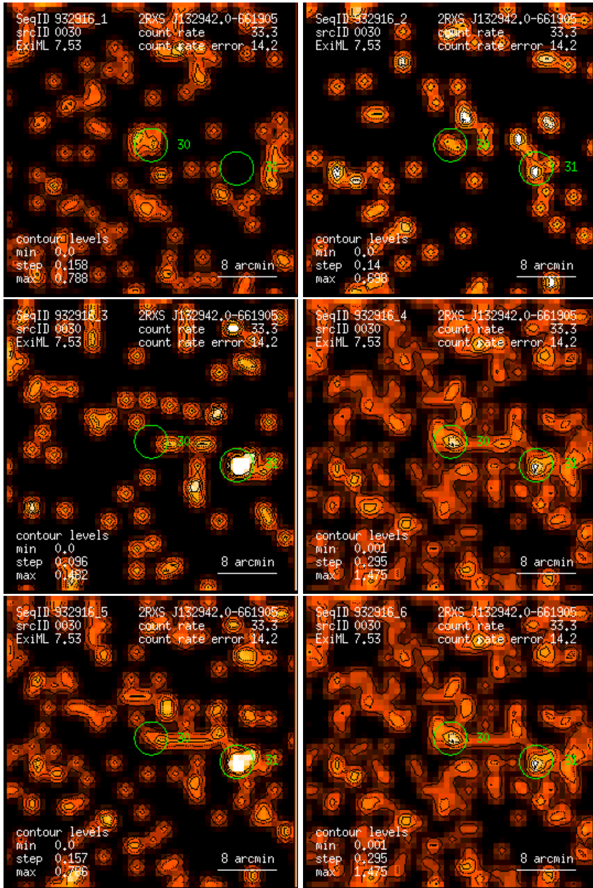
Figure 30: RASS 932916: detection 0030: band rate images, Gaussian filter: (1) PSPC channels 11 – 41, (2) 52 – 90, (3) 91 – 201, (4) 11 – 235, (5) 52 – 201, (6) 11 – 201. Broad band rates in counts/ks. Band rate contour levels in counts/ks/arcmin 2 .
