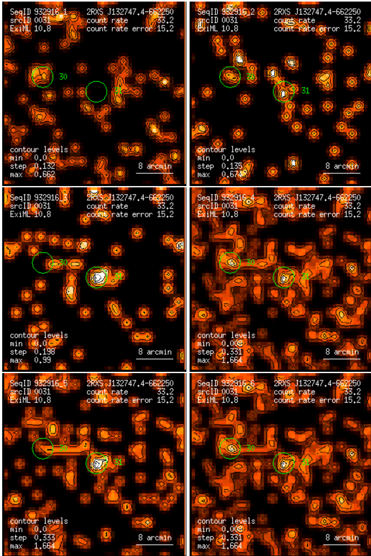
Figure 31: RASS 932916: detection 0031: band rate images, Gaussian filter: (1) PSPC channels 11 – 41, (2) 52 – 90, (3) 91 – 201, (4) 11 – 235, (5) 52 – 201, (6) 11 – 201. Broad band rates in counts/ks. Band rate contour levels in counts/ks/arcmin 2 .
