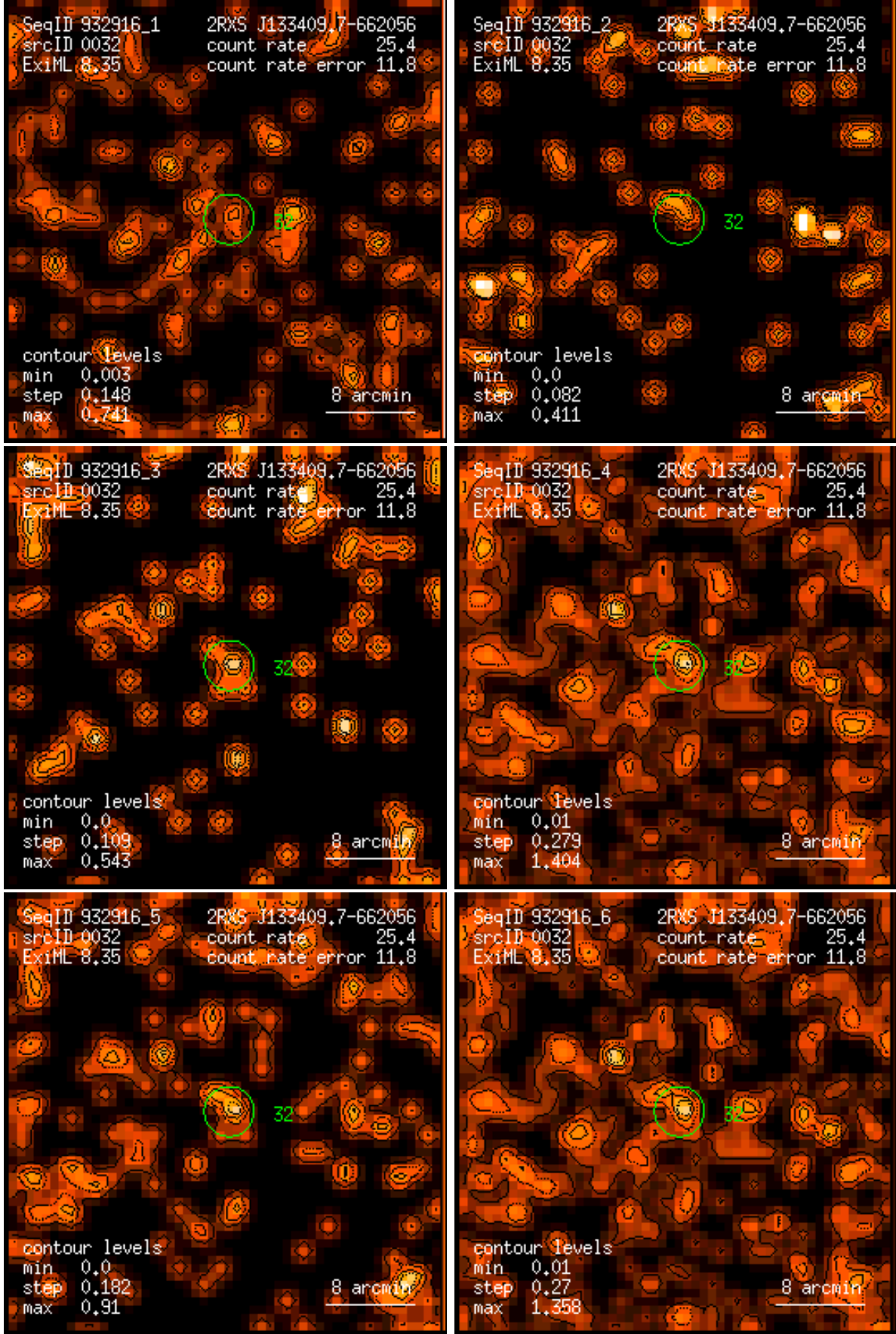
Figure 32: RASS 932916: detection 0032: band rate images, Gaussian filter: (1) PSPC channels 11 – 41, (2) 52 – 90, (3) 91 – 201, (4) 11 – 235, (5) 52 – 201, (6) 11 – 201. Broad band rates in counts/ks. Band rate contour levels in counts/ks/arcmin 2 .
