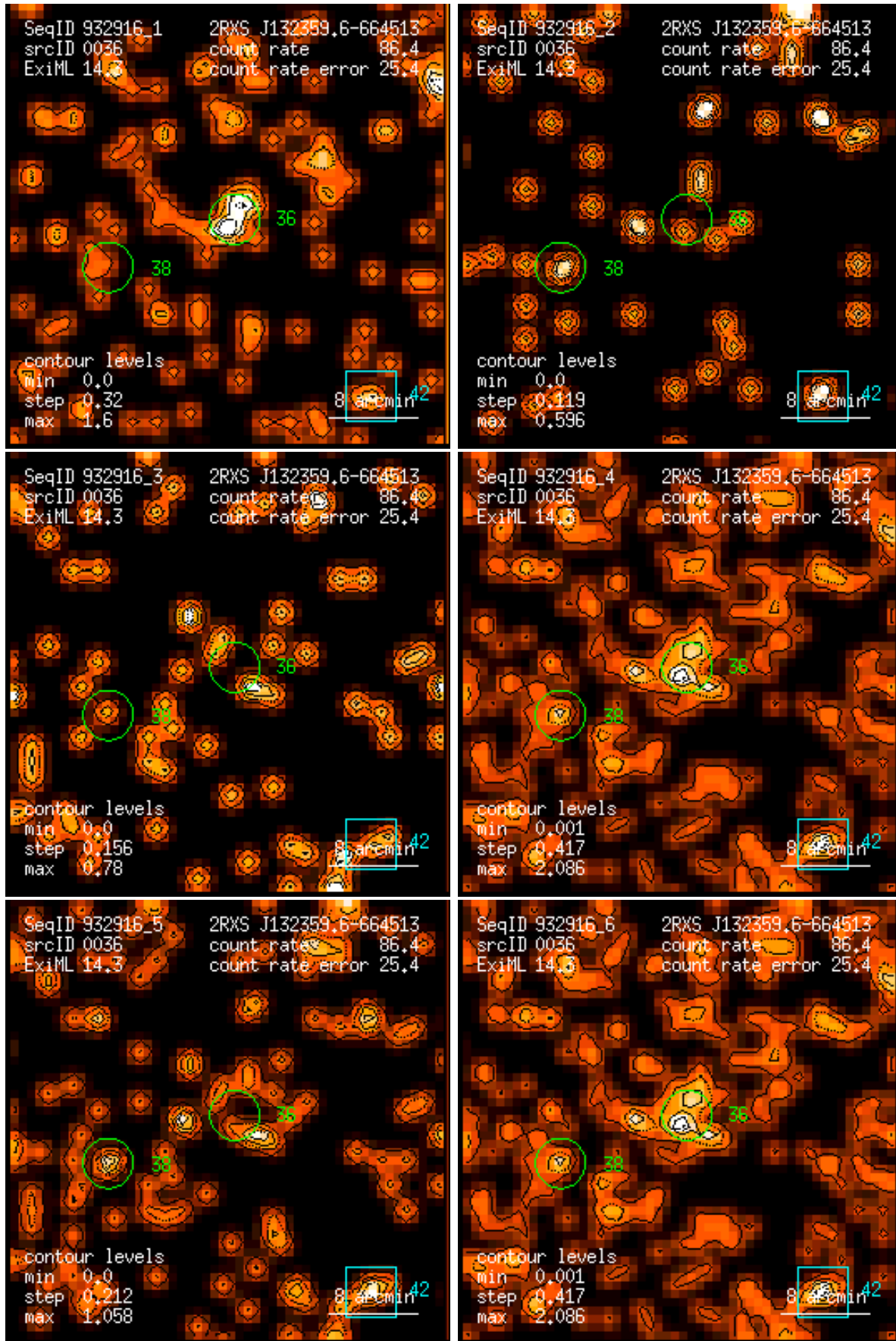
Figure 36: RASS 932916: detection 0036: band rate images, Gaussian filter: (1) PSPC channels 11 – 41, (2) 52 – 90, (3) 91 – 201, (4) 11 – 235, (5) 52 – 201, (6) 11 – 201. Broad band rates in counts/ks. Band rate contour levels in counts/ks/arcmin 2 .
