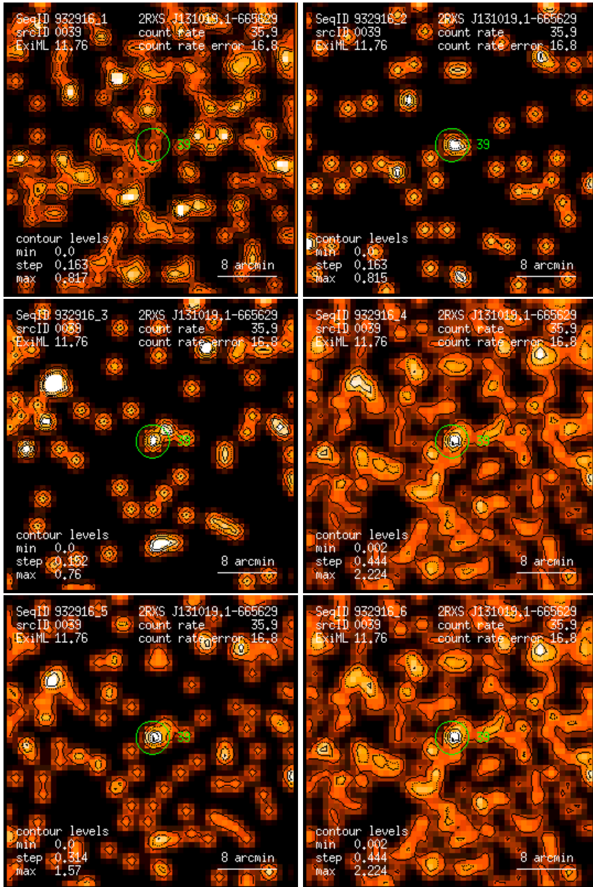
Figure 39: RASS 932916: detection 0039: band rate images, Gaussian filter: (1) PSPC channels 11 – 41, (2) 52 – 90, (3) 91 – 201, (4) 11 – 235, (5) 52 – 201, (6) 11 – 201. Broad band rates in counts/ks. Band rate contour levels in counts/ks/arcmin 2 .
