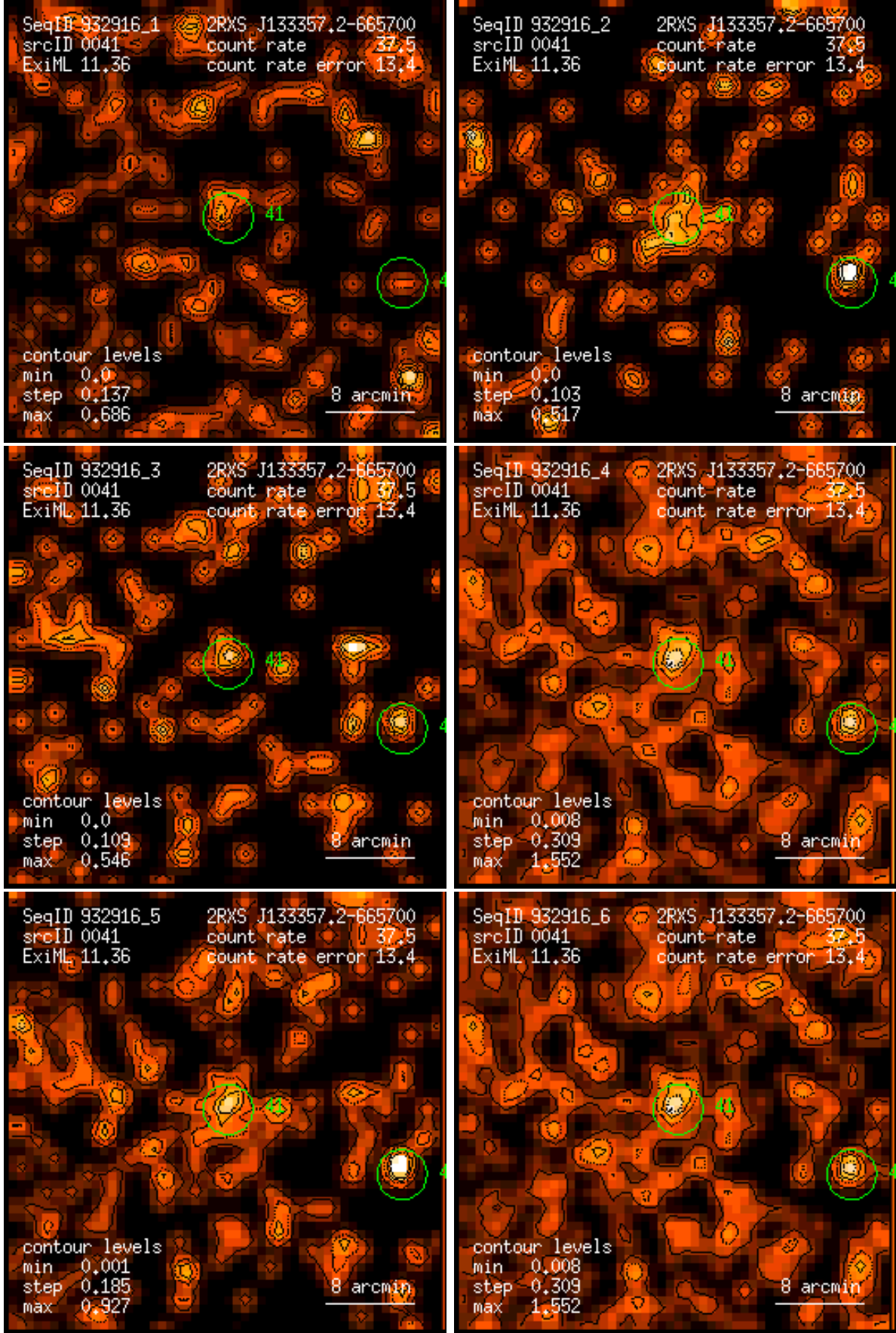
Figure 41: RASS 932916: detection 0041: band rate images, Gaussian filter: (1) PSPC channels 11 – 41, (2) 52 – 90, (3) 91 – 201, (4) 11 – 235, (5) 52 – 201, (6) 11 – 201. Broad band rates in counts/ks. Band rate contour levels in counts/ks/arcmin 2 .
