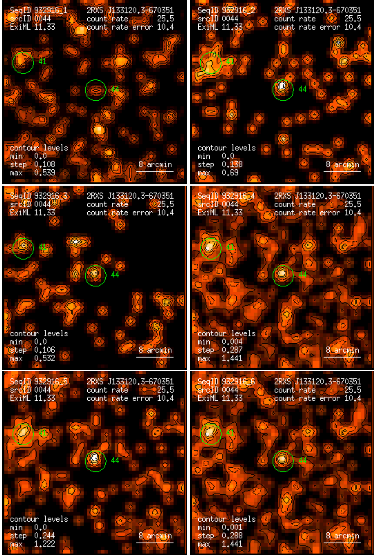
Figure 44: RASS 932916: detection 0044: band rate images, Gaussian filter: (1) PSPC channels 11 – 41, (2) 52 – 90, (3) 91 – 201, (4) 11 – 235, (5) 52 – 201, (6) 11 – 201. Broad band rates in counts/ks. Band rate contour levels in counts/ks/arcmin 2 .
