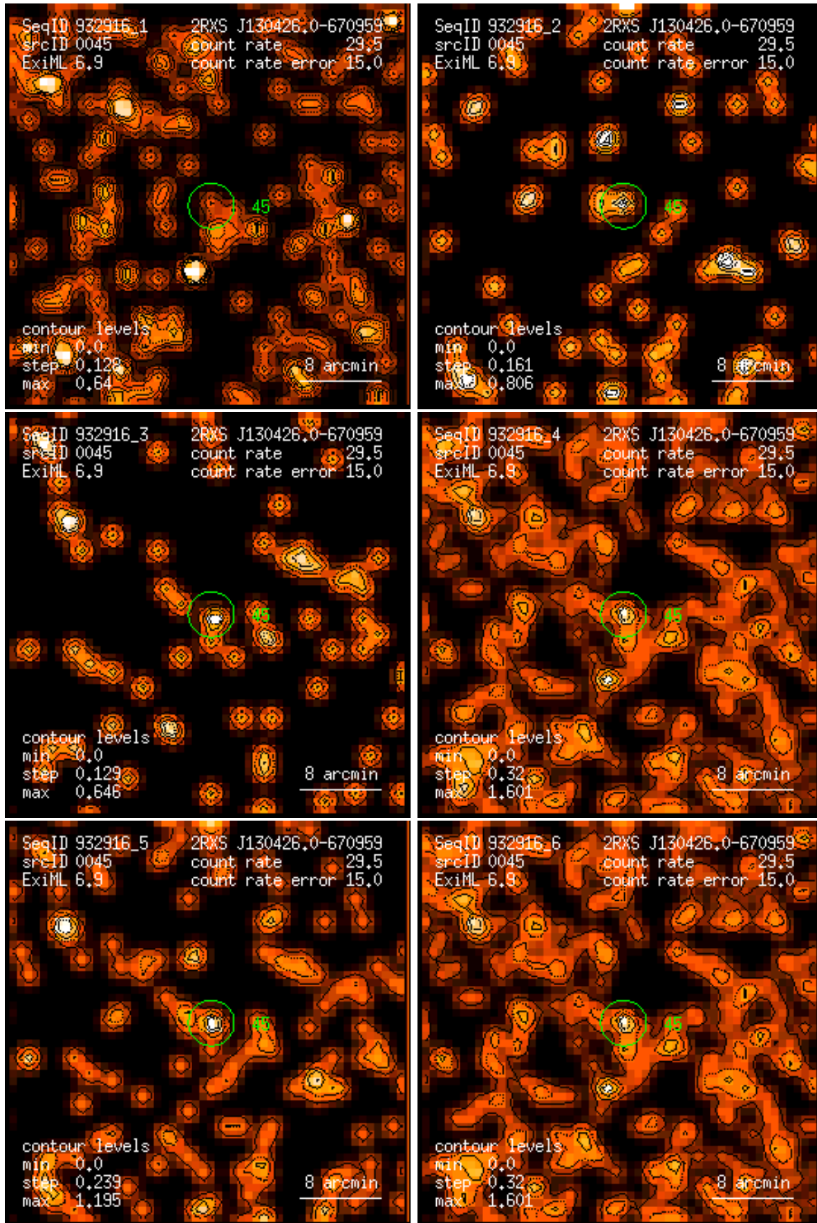
Figure 45: RASS 932916: detection 0045: band rate images, Gaussian filter: (1) PSPC channels 11 – 41, (2) 52 – 90, (3) 91 – 201, (4) 11 – 235, (5) 52 – 201, (6) 11 – 201. Broad band rates in counts/ks. Band rate contour levels in counts/ks/arcmin 2 .
