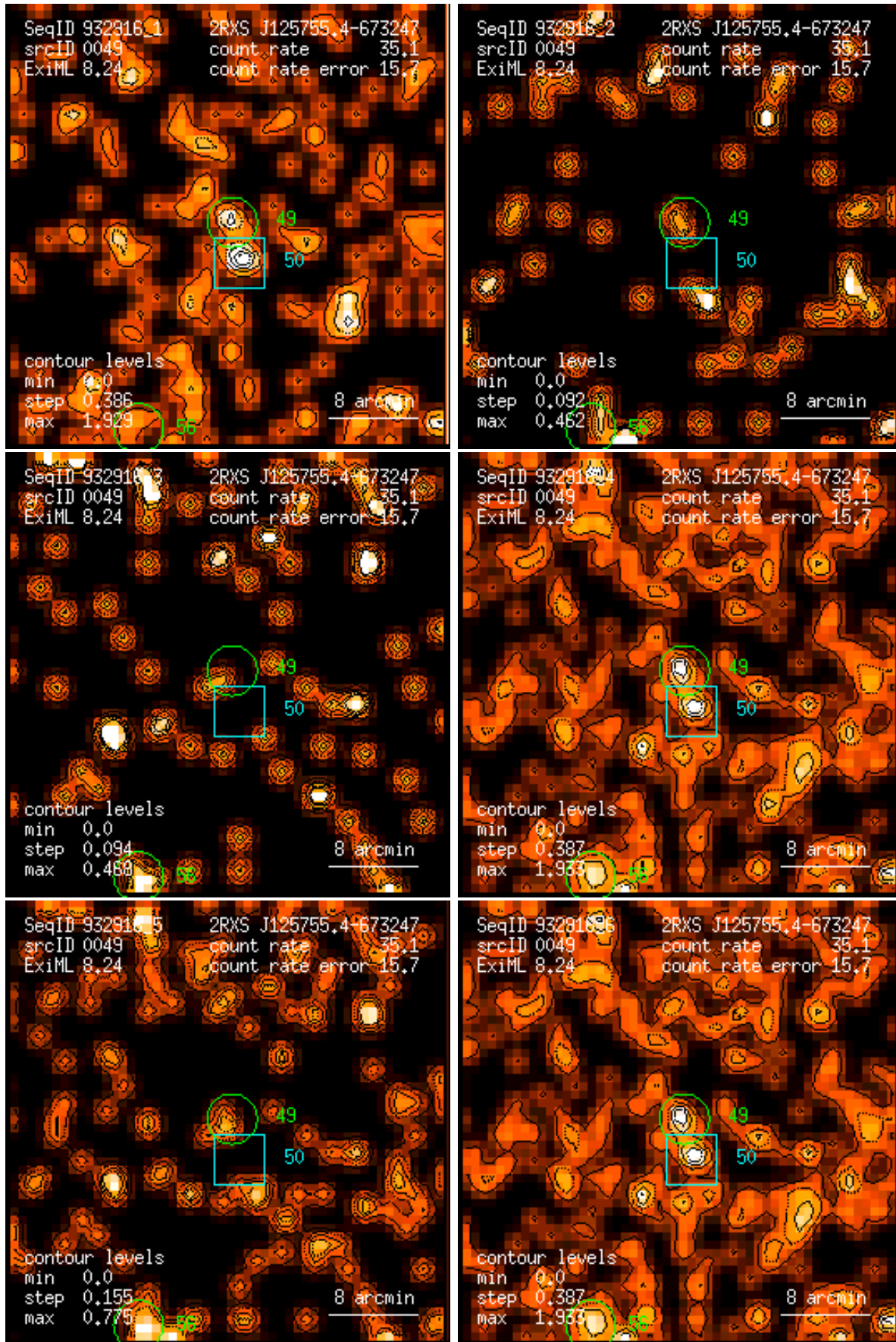
Figure 49: RASS 932916: detection 0049: band rate images, Gaussian filter: (1) PSPC channels 11 – 41, (2) 52 – 90, (3) 91 – 201, (4) 11 – 235, (5) 52 – 201, (6) 11 – 201. Broad band rates in counts/ks. Band rate contour levels in counts/ks/arcmin 2 .
