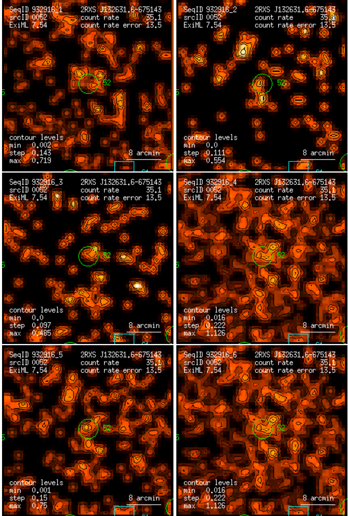
Figure 52: RASS 932916: detection 0052: band rate images, Gaussian filter: (1) PSPC channels 11 – 41, (2) 52 – 90, (3) 91 – 201, (4) 11 – 235, (5) 52 – 201, (6) 11 – 201. Broad band rates in counts/ks. Band rate contour levels in counts/ks/arcmin 2 .
