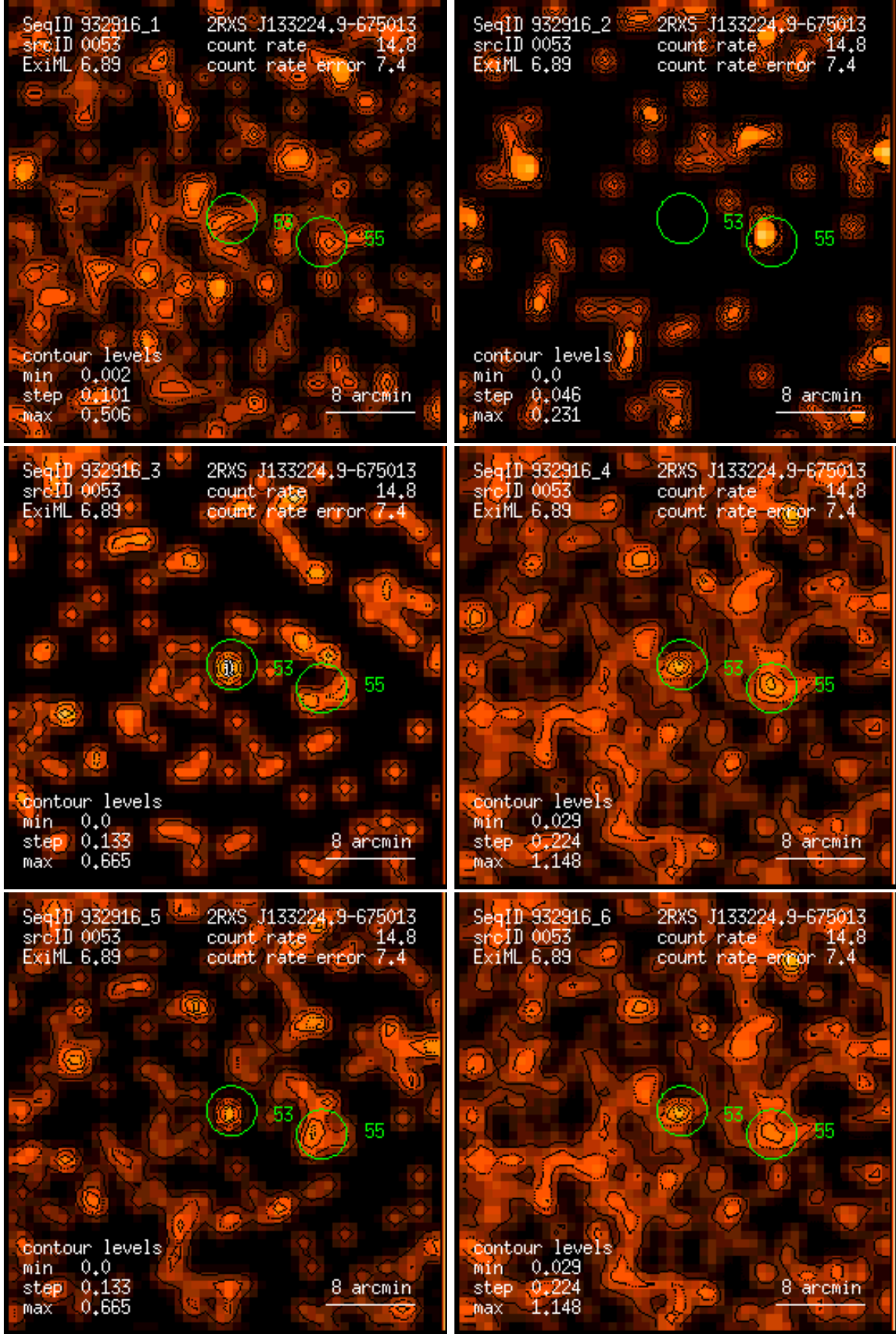
Figure 53: RASS 932916: detection 0053: band rate images, Gaussian filter: (1) PSPC channels 11 – 41, (2) 52 – 90, (3) 91 – 201, (4) 11 – 235, (5) 52 – 201, (6) 11 – 201. Broad band rates in counts/ks. Band rate contour levels in counts/ks/arcmin 2 .
