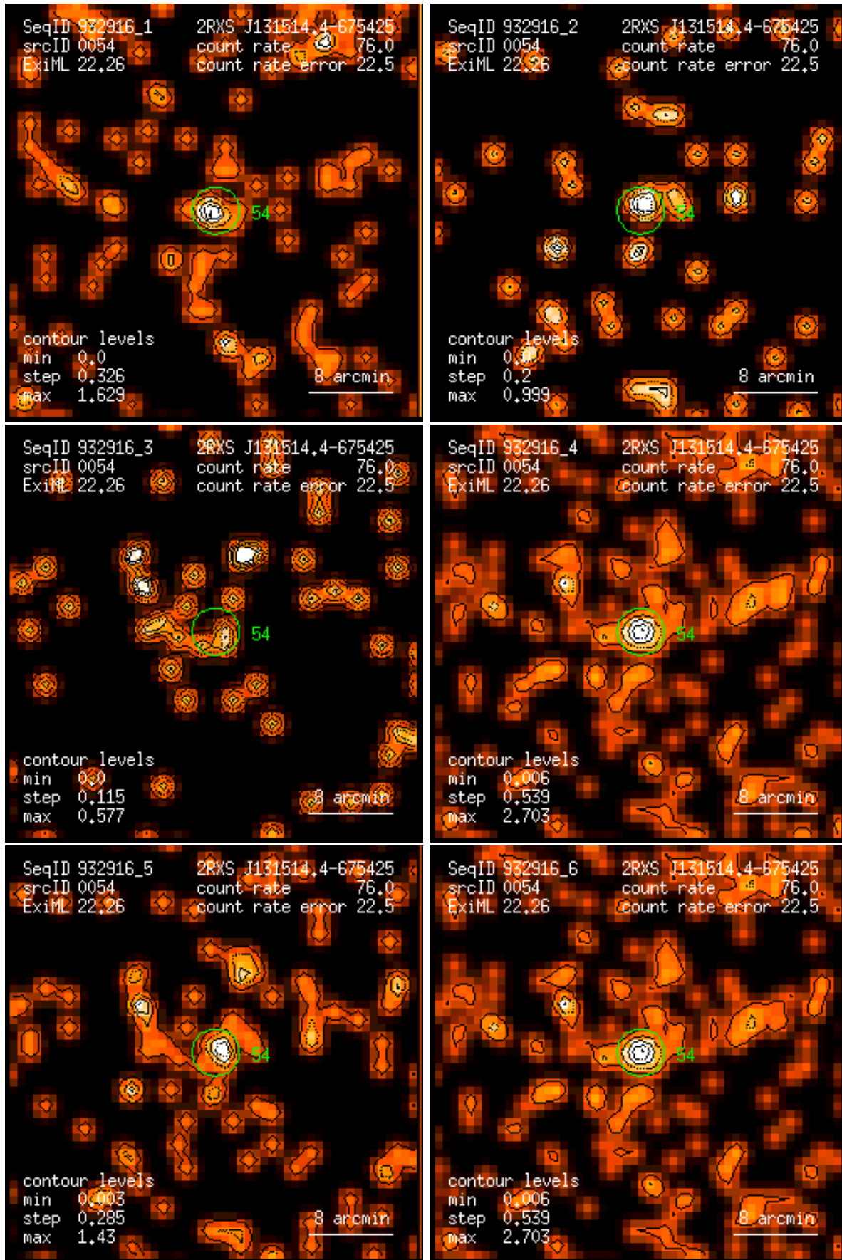
Figure 54: RASS 932916: detection 0054: band rate images, Gaussian filter: (1) PSPC channels 11 – 41, (2) 52 – 90, (3) 91 – 201, (4) 11 – 235, (5) 52 – 201, (6) 11 – 201. Broad band rates in counts/ks. Band rate contour levels in counts/ks/arcmin 2 .
