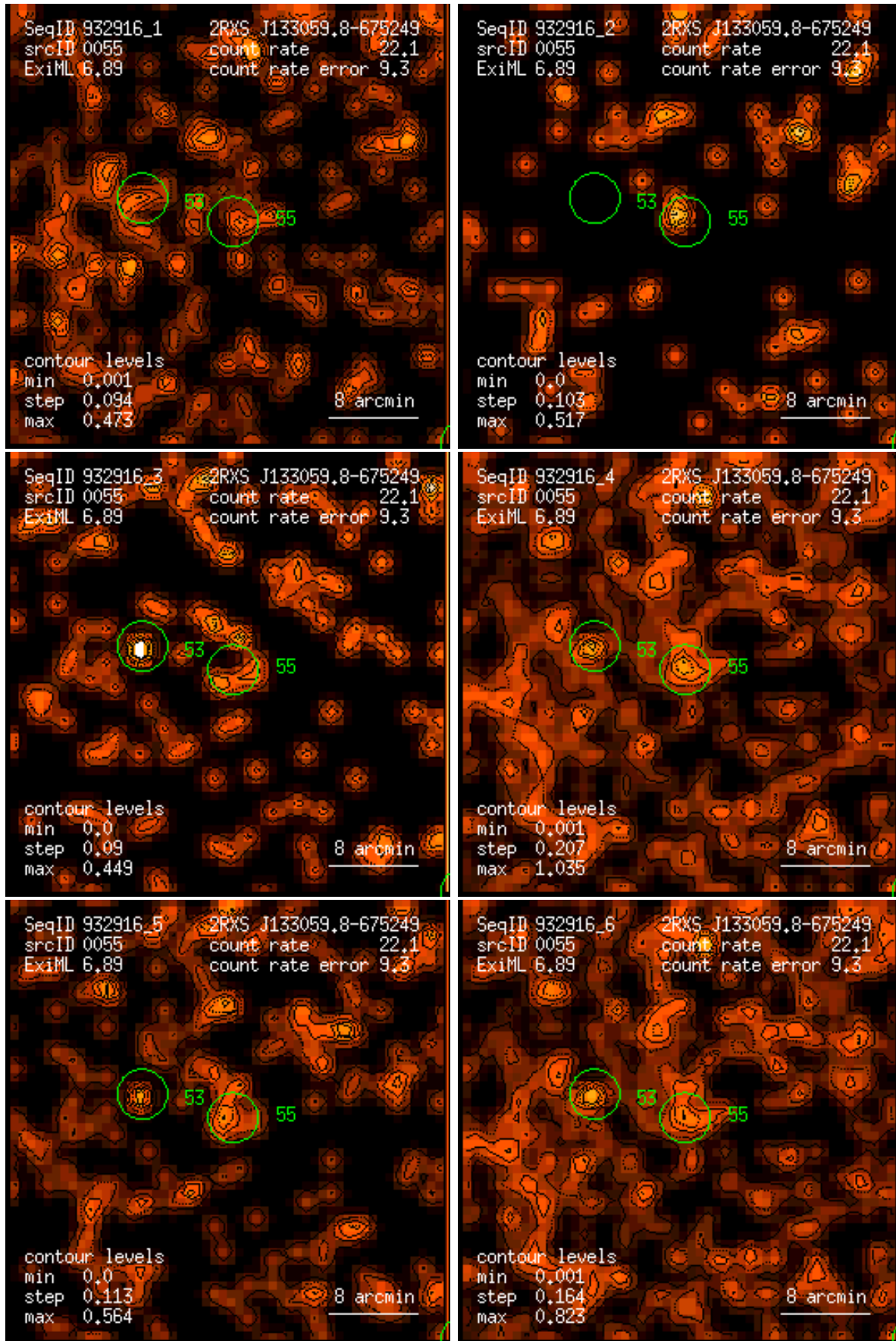
Figure 55: RASS 932916: detection 0055: band rate images, Gaussian filter: (1) PSPC channels 11 – 41, (2) 52 – 90, (3) 91 – 201, (4) 11 – 235, (5) 52 – 201, (6) 11 – 201. Broad band rates in counts/ks. Band rate contour levels in counts/ks/arcmin 2 .
