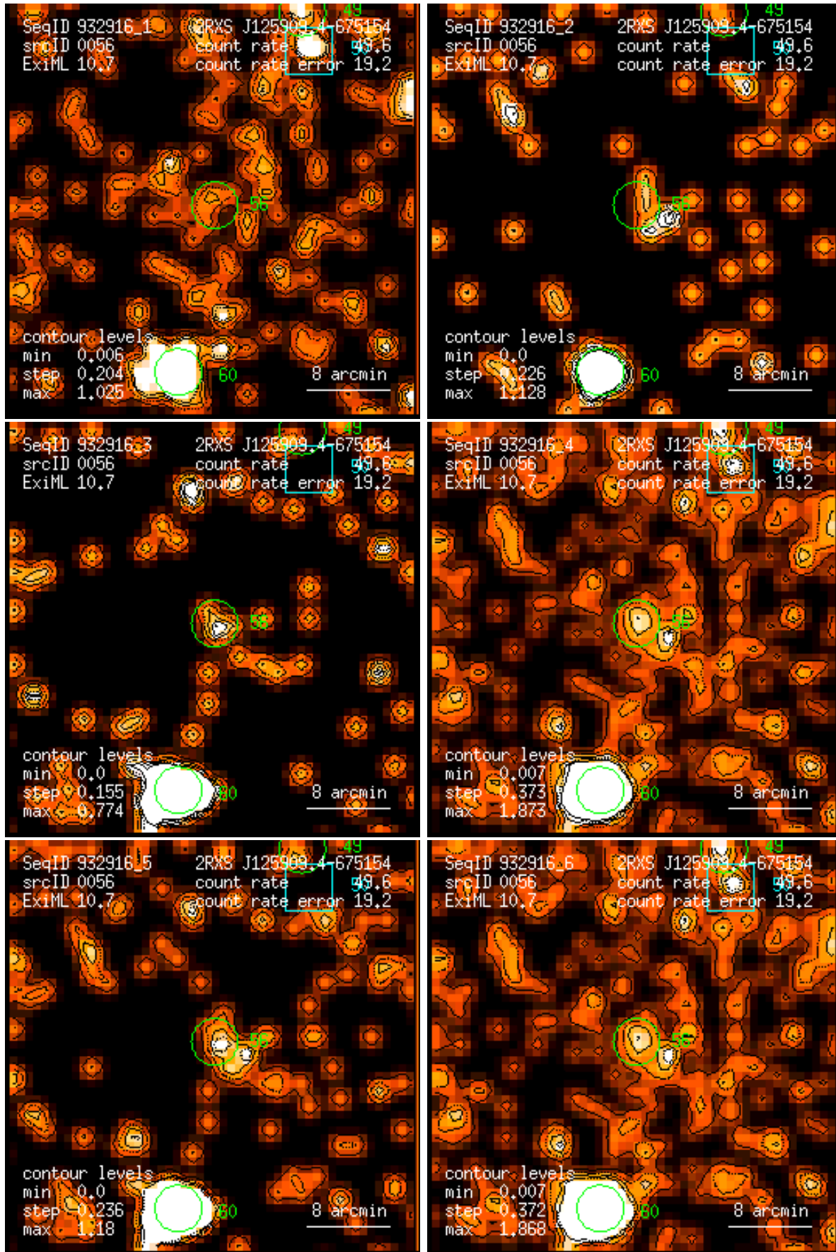
Figure 56: RASS 932916: detection 0056: band rate images, Gaussian filter: (1) PSPC channels 11 – 41, (2) 52 – 90, (3) 91 – 201, (4) 11 – 235, (5) 52 – 201, (6) 11 – 201. Broad band rates in counts/ks. Band rate contour levels in counts/ks/arcmin 2 .
