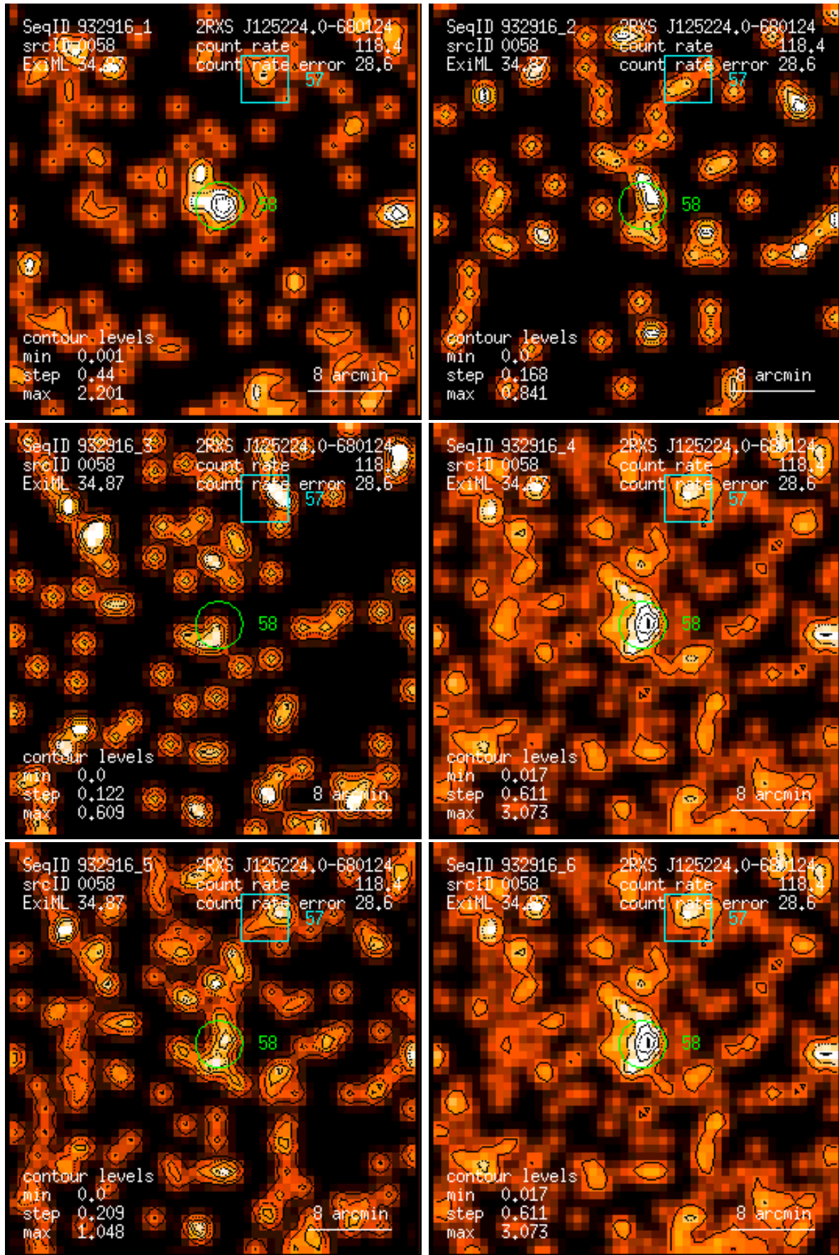
Figure 58: RASS 932916: detection 0058: band rate images, Gaussian filter: (1) PSPC channels 11 – 41, (2) 52 – 90, (3) 91 – 201, (4) 11 – 235, (5) 52 – 201, (6) 11 – 201. Broad band rates in counts/ks. Band rate contour levels in counts/ks/arcmin 2 .
