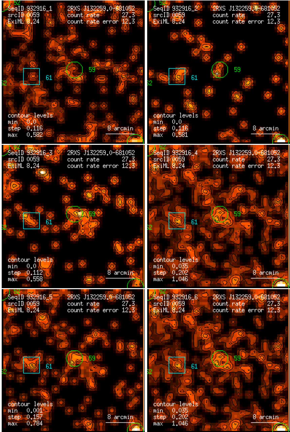
Figure 59: RASS 932916: detection 0059: band rate images, Gaussian filter: (1) PSPC channels 11 – 41, (2) 52 – 90, (3) 91 – 201, (4) 11 – 235, (5) 52 – 201, (6) 11 – 201. Broad band rates in counts/ks. Band rate contour levels in counts/ks/arcmin 2 .
