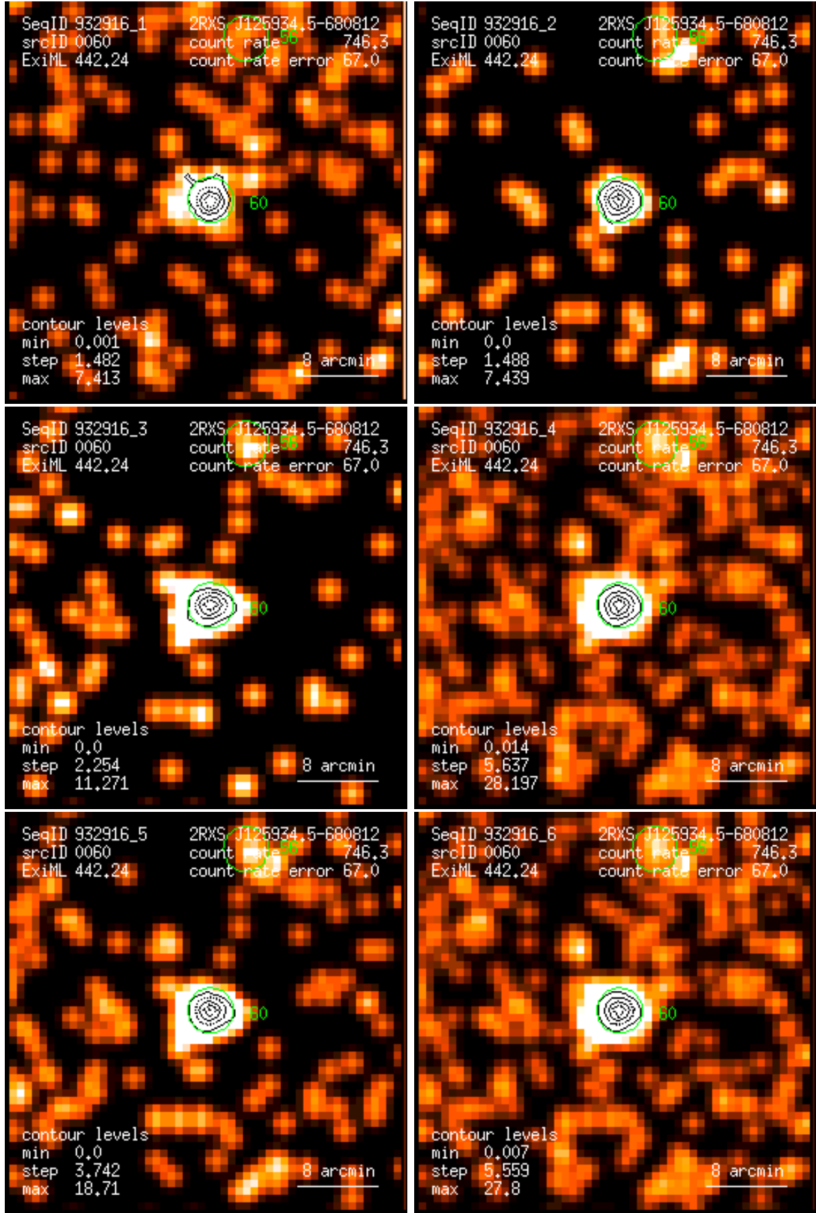
Figure 60: RASS 932916: detection 0060: band rate images, Gaussian filter: (1) PSPC channels 11 – 41, (2) 52 – 90, (3) 91 – 201, (4) 11 – 235, (5) 52 – 201, (6) 11 – 201. Broad band rates in counts/ks. Band rate contour levels in counts/ks/arcmin 2 .
