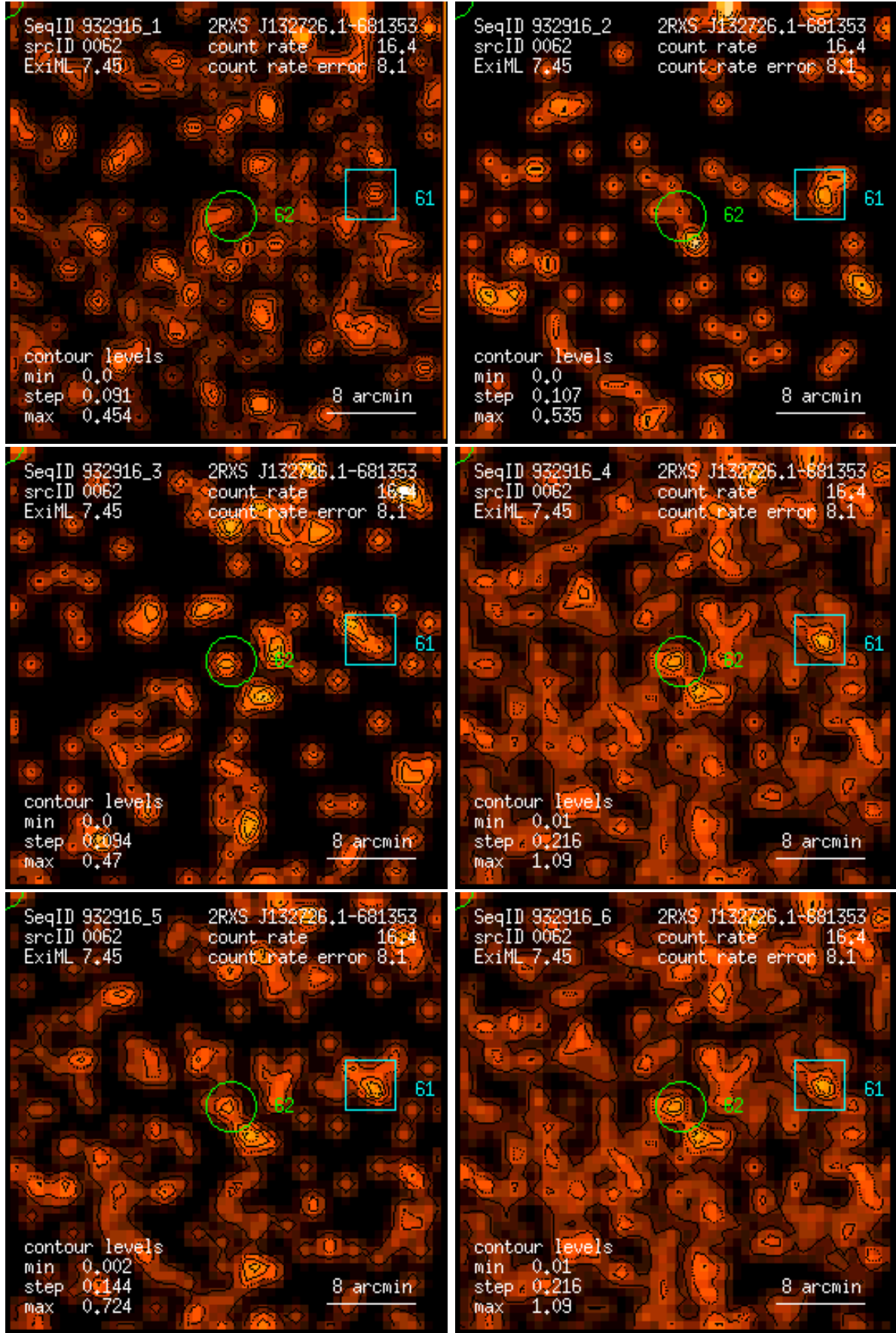
Figure 62: RASS 932916: detection 0062: band rate images, Gaussian filter: (1) PSPC channels 11 – 41, (2) 52 – 90, (3) 91 – 201, (4) 11 – 235, (5) 52 – 201, (6) 11 – 201. Broad band rates in counts/ks. Band rate contour levels in counts/ks/arcmin 2 .
