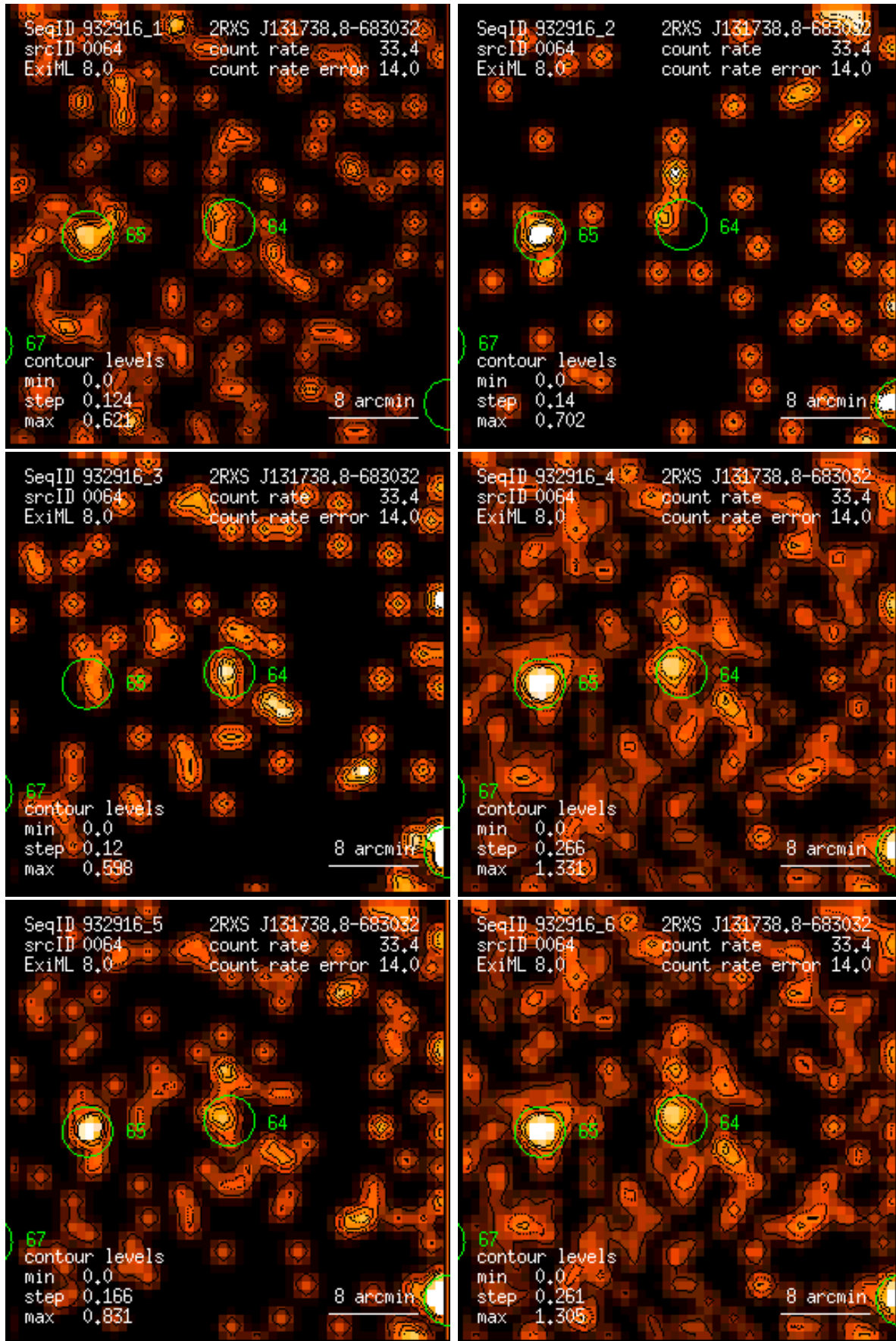
Figure 64: RASS 932916: detection 0064: band rate images, Gaussian filter: (1) PSPC channels 11 – 41, (2) 52 – 90, (3) 91 – 201, (4) 11 – 235, (5) 52 – 201, (6) 11 – 201. Broad band rates in counts/ks. Band rate contour levels in counts/ks/arcmin 2 .
