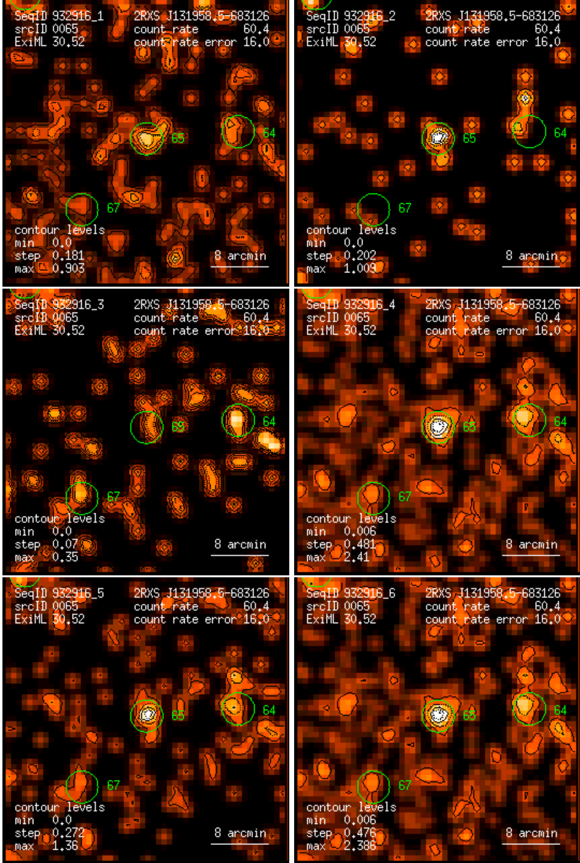
Figure 65: RASS 932916: detection 0065: band rate images, Gaussian filter: (1) PSPC channels 11 – 41, (2) 52 – 90, (3) 91 – 201, (4) 11 – 235, (5) 52 – 201, (6) 11 – 201. Broad band rates in counts/ks. Band rate contour levels in counts/ks/arcmin 2 .
