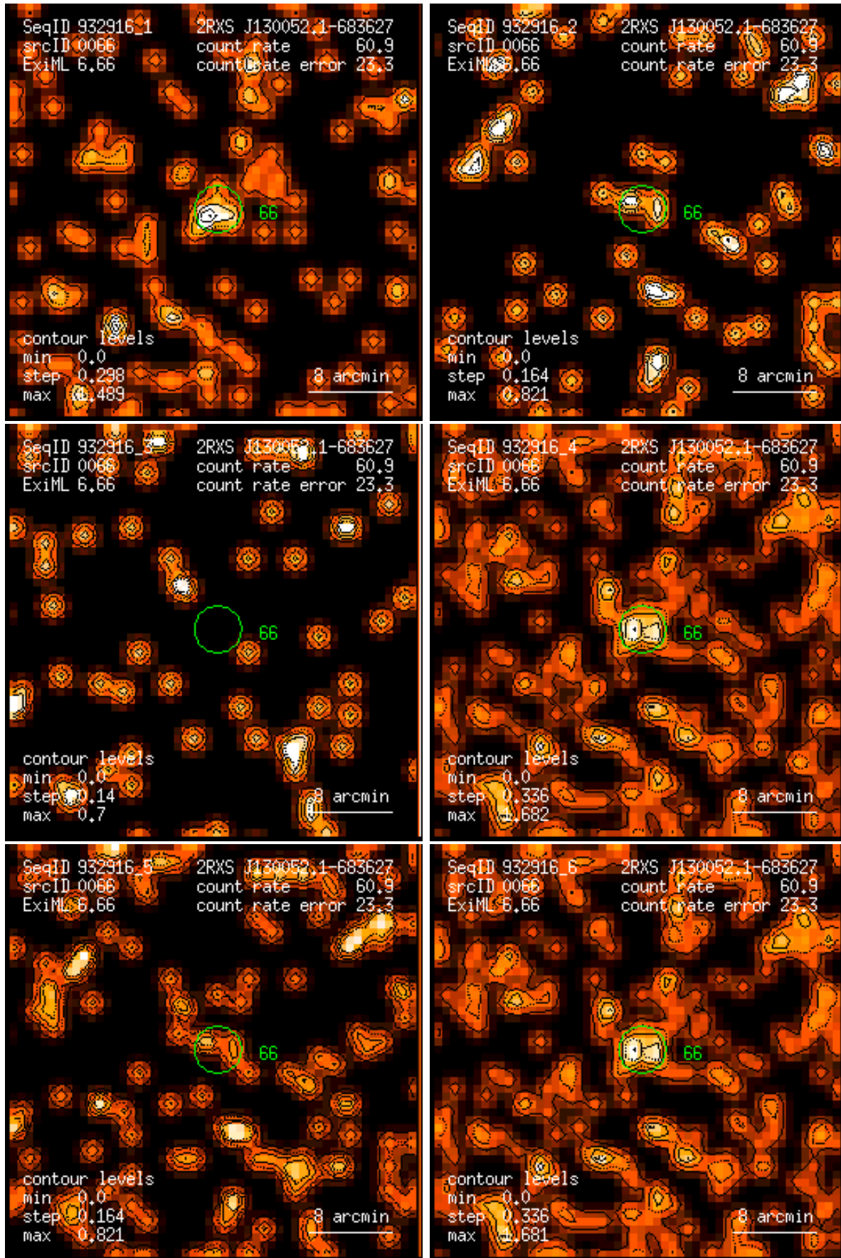
Figure 66: RASS 932916: detection 0066: band rate images, Gaussian filter: (1) PSPC channels 11 – 41, (2) 52 – 90, (3) 91 – 201, (4) 11 – 235, (5) 52 – 201, (6) 11 – 201. Broad band rates in counts/ks. Band rate contour levels in counts/ks/arcmin 2 .
