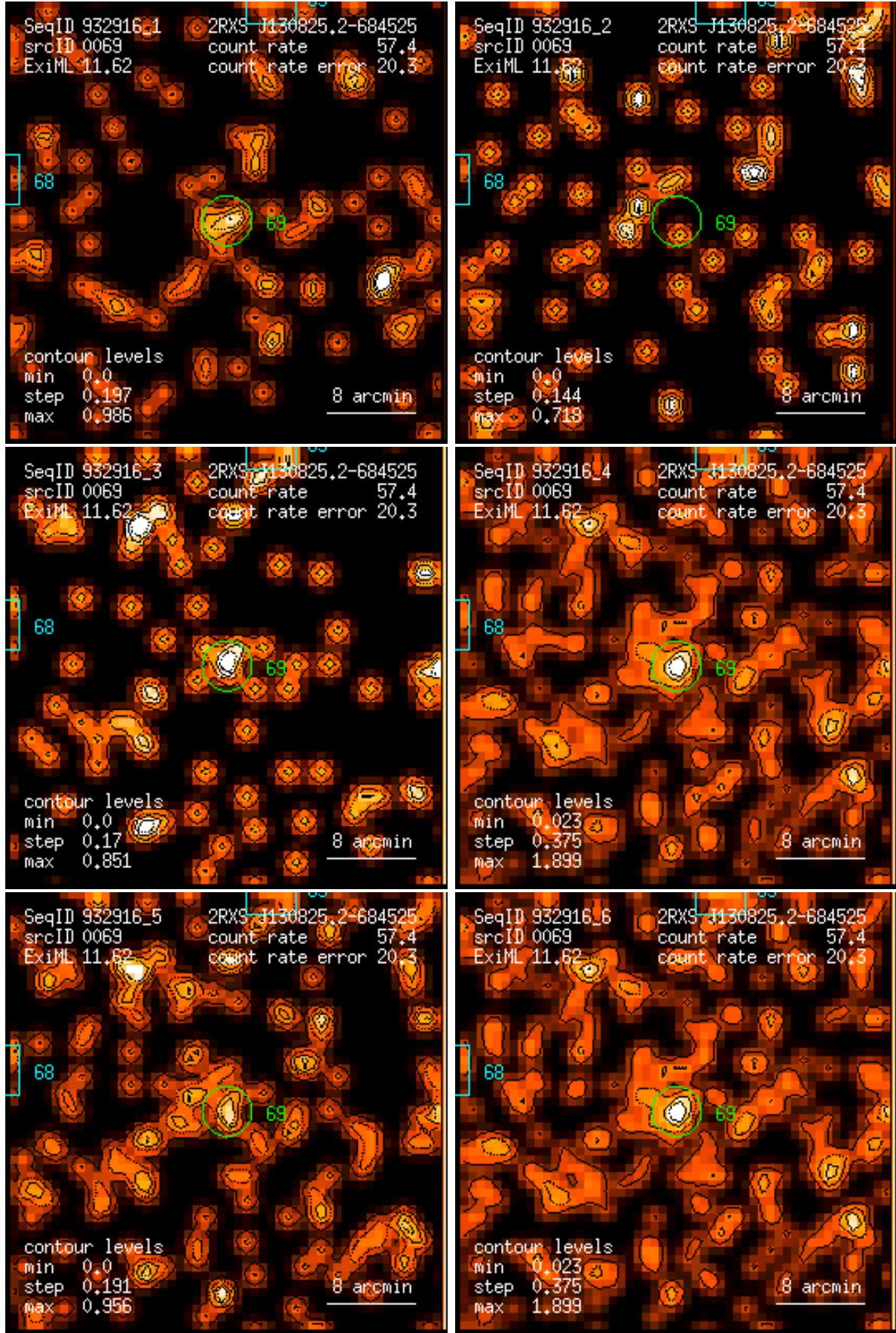
Figure 69: RASS 932916: detection 0069: band rate images, Gaussian filter: (1) PSPC channels 11 – 41, (2) 52 – 90, (3) 91 – 201, (4) 11 – 235, (5) 52 – 201, (6) 11 – 201. Broad band rates in counts/ks. Band rate contour levels in counts/ks/arcmin 2 .
