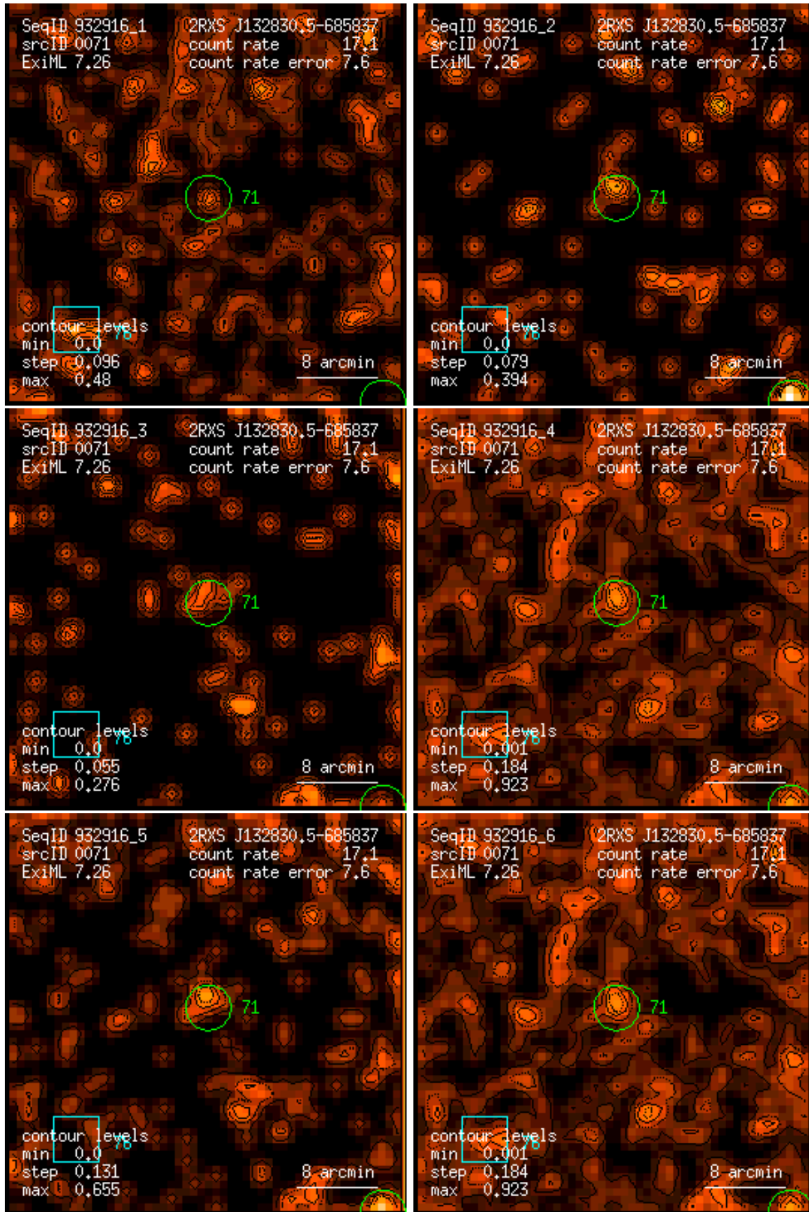
Figure 71: RASS 932916: detection 0071: band rate images, Gaussian filter: (1) PSPC channels 11 – 41, (2) 52 – 90, (3) 91 – 201, (4) 11 – 235, (5) 52 – 201, (6) 11 – 201. Broad band rates in counts/ks. Band rate contour levels in counts/ks/arcmin 2 .
