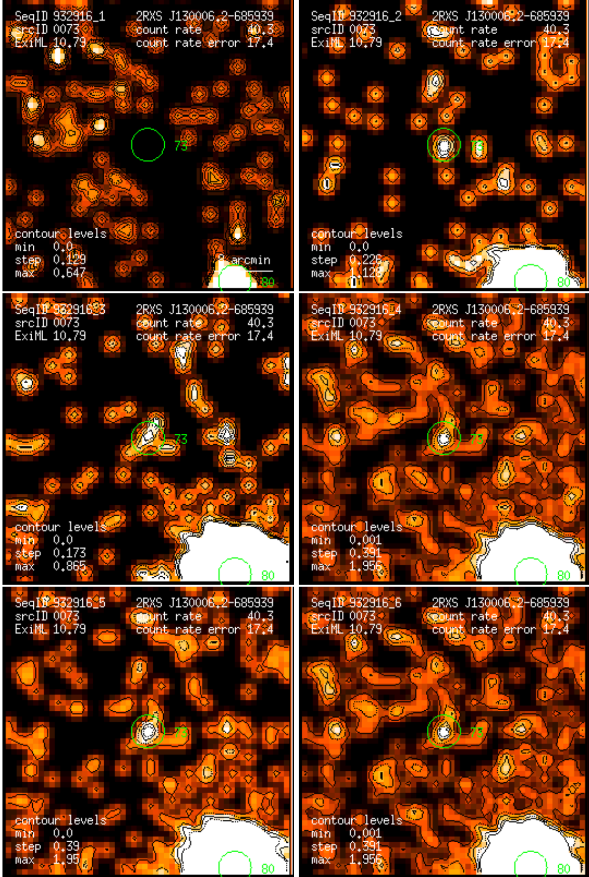
Figure 73: RASS 932916: detection 0073: band rate images, Gaussian filter: (1) PSPC channels 11 – 41, (2) 52 – 90, (3) 91 – 201, (4) 11 – 235, (5) 52 – 201, (6) 11 – 201. Broad band rates in counts/ks. Band rate contour levels in counts/ks/arcmin 2 .
