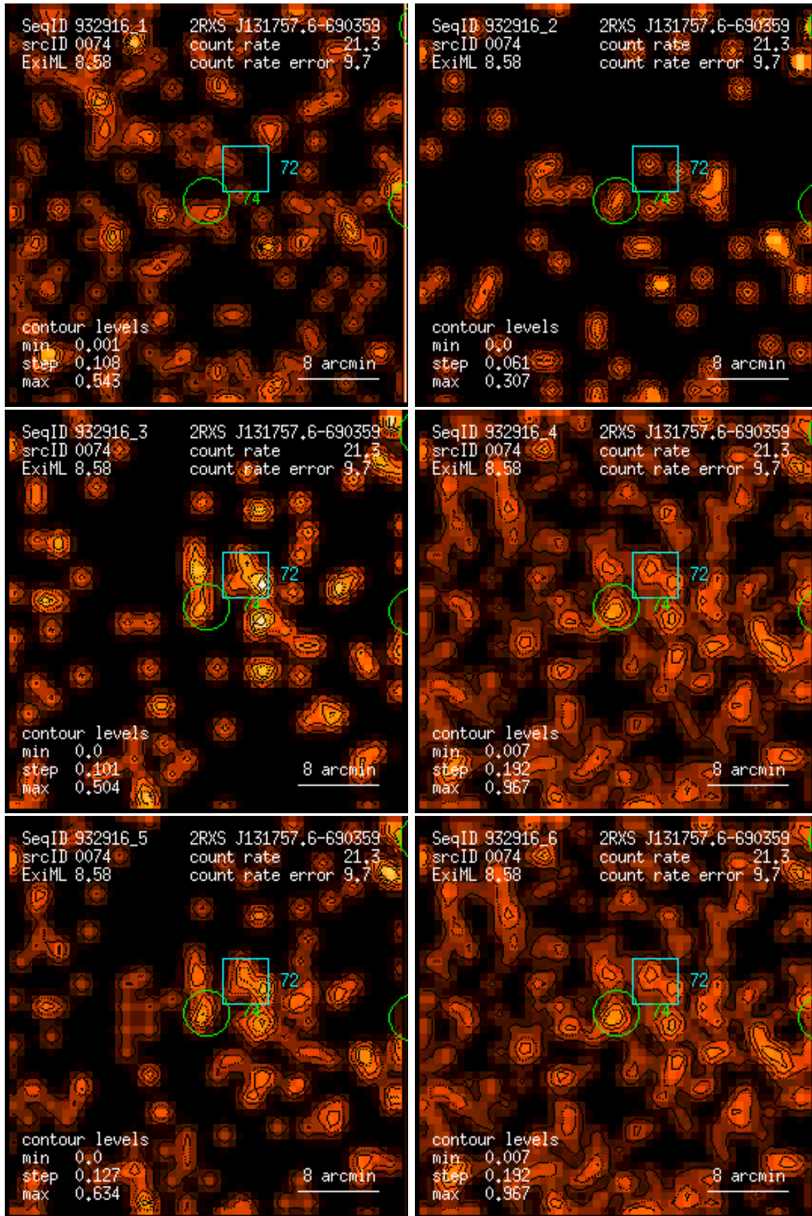
Figure 74: RASS 932916: detection 0074: band rate images, Gaussian filter: (1) PSPC channels 11 – 41, (2) 52 – 90, (3) 91 – 201, (4) 11 – 235, (5) 52 – 201, (6) 11 – 201. Broad band rates in counts/ks. Band rate contour levels in counts/ks/arcmin 2 .
